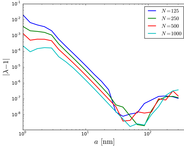
Figure 59: Difference between the leading eigenvalue of the operator \mathcal{K} ( \lambda_1 ) and the leading eigenvalue of the matrix representation of this operator after discretization, as a function of grain size for different numerical resolutions.
