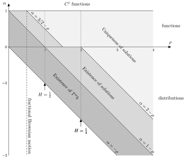
FIGURE 1.1 – Averaging ODE for \rho -irregular perturbations
