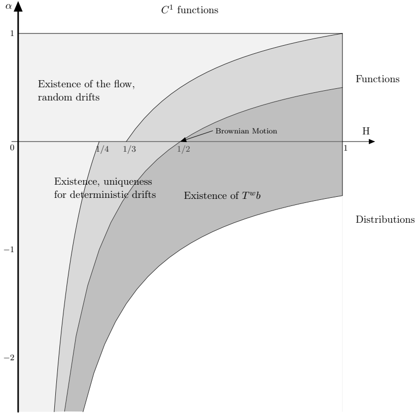
FIGURE 1.2 – Averaging ODE for fractional Brownian motion
