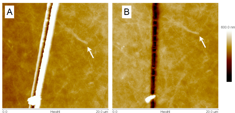
Figure 92. AFM images of the cut made in a (MFC/PVAm) 30 film (1.65 \mu\text{m} thick) before immersion in water (A) and after immersion in water for five minutes and drying (B). A random feature in the film, indicated by the white arrow, confirms that both images were taken at the same location.
