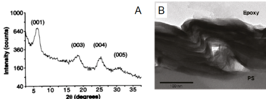
Figure 31. Clay-containing multilayers. (A) X-ray diffractogram of a multilayer showing multiple reflections due to regular basal spacing (1.5 nm). 101 (B) TEM cross-section micrograph of a clay-containing multilayer. 122
