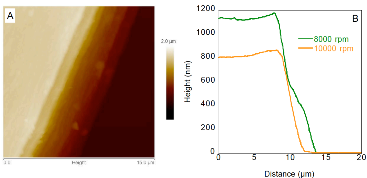
Figure 94. (A) AFM image of the edge of a (PVAm/MFC) 200 film assembled by spin-assisted LbL with a rotation speed of 8000rpm resting on a silicon wafer. (B) Profiles measured on the AFM images for (PVAm/MFC) 200 assembled with a rotation speed of 8000 rpm, and (PVAm/MFC) 120 assembled with a rotation speed of 10000 rpm.
