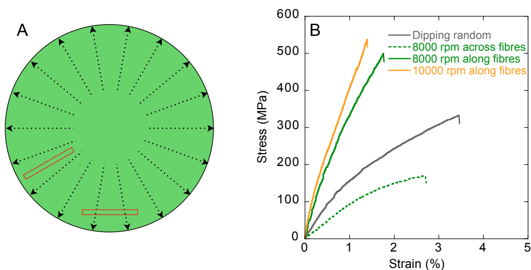
Figure 98. (A) Schematic representation of the sample preparation for the mechanical tests. The arrows indicate the directions of orientation of the fibers and the red lines the edges of the samples (parallel and perpendicular to the direction of orientation). (B) Typical stress strain curves obtained for (PVAm/MFC) films prepared by dipping (not oriented) and spin-assisted assembly (oriented). The rotation speed during spin-assisted assembly is reported together with the direction of solicitation.
