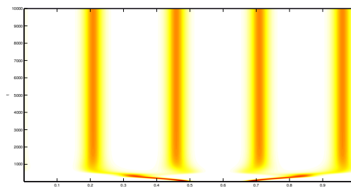
FIGURE B.5 – Numerical population density dynamics obtained by deterministic simulations for model (B.7)–(B.12) with periodic boundary conditions. We have used the following parameter values : \lambda = 0.001 , \sigma = 0.04 , \Delta t = 0.0001 , \Delta x = 0.001 , L = 1 , N = 1000 .
