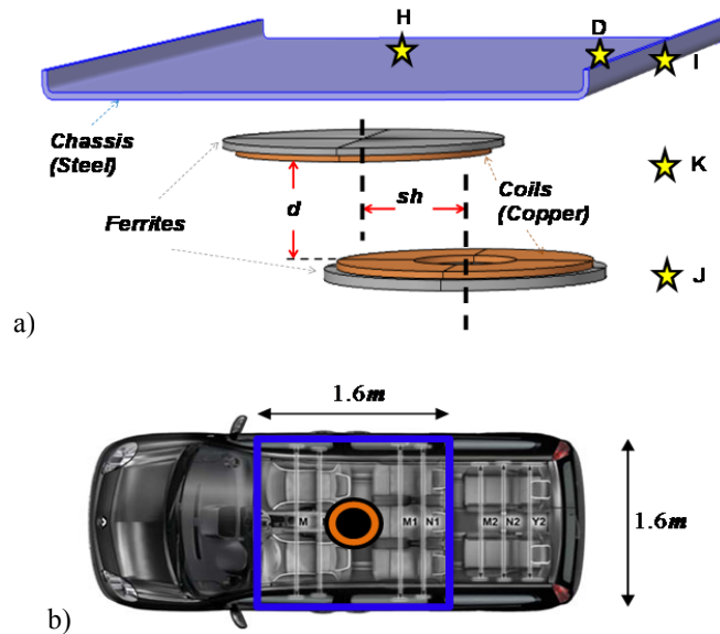
Fig. IV.2: a) 3D structure of an ICT with shielding, simple EV chassis and measurement positions (stars) for the magnetic field density, b) top view of the EV to show the considered chassis and the position of secondary pad
