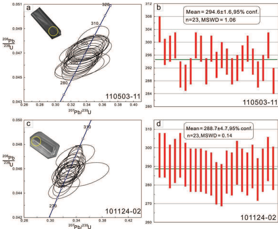
图5-22 克什克腾旗南清风山组双峰式火山岩年龄: a 和 b, 玄武安山岩; c 和 d, 流纹岩 Figure 5-22 U-Pb zircon geochronology results of Qingfengshan Formation bimodal volcanic rocks in Keshiketengqi area: a and b, basaltic andesite; c and d, rhyolite
