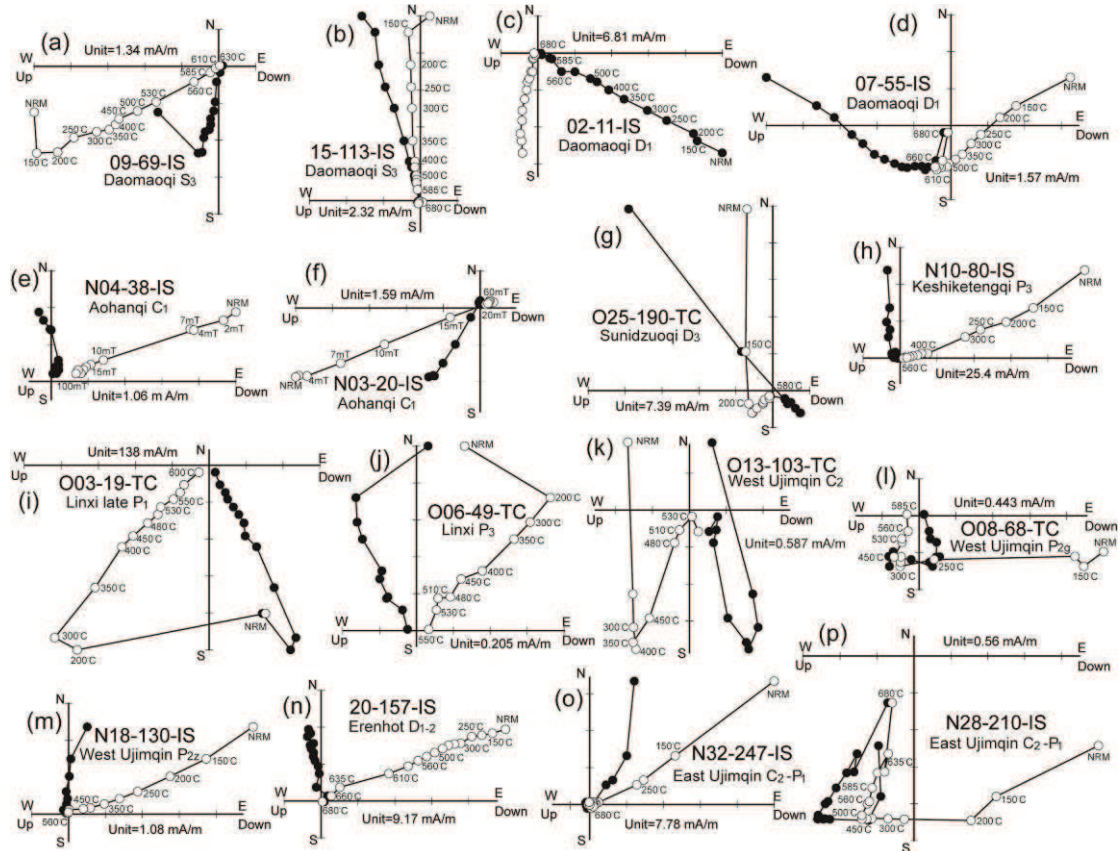
Figure 6-5 Orthogonal vector plots of representative specimens from each sampled age/locality group. Closed (open) symbols present the projection in horizontal (vertical) plane. IS (in-situ) and TC (tilt-corrected) stands for plot in in-situ and tilt-corrected coordinates. Sample name, site locality and stratigraphic age are shown on each figure.
