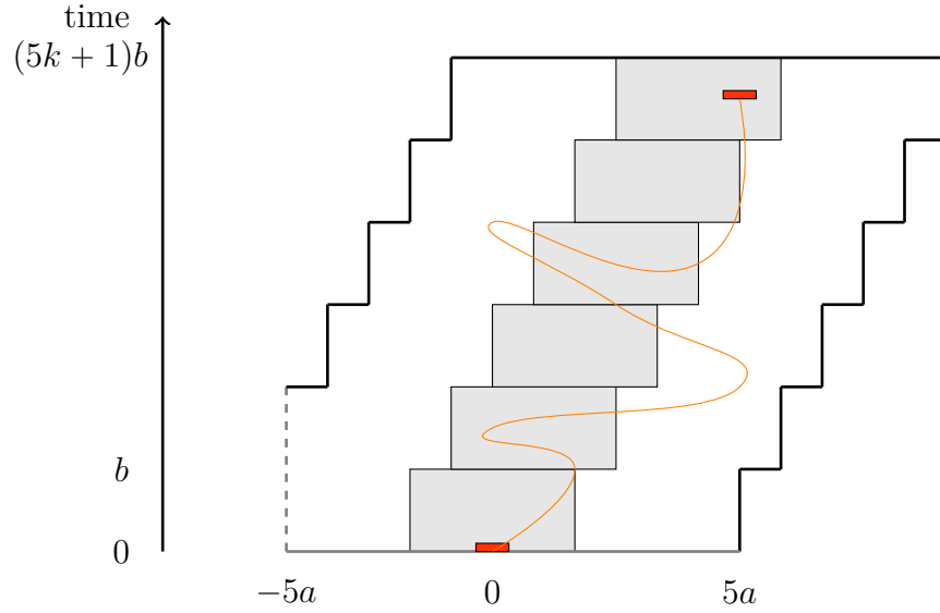
FIGURE 2.3: Set d = 1 . The targeted region goes upward-rightward (reflections are not drawn, but a symmetric draw going upward-leftward does exist as the dashed line suggests it). Occupied translated sets [-n, n]^d stand in the gray regions and are reached by paths lying in the area delimited by the stair shaped plain lines.
