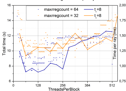
Figure 5: Search for the best performance (8,100 rays)
