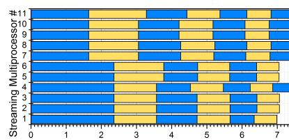
Figure 9: Variable size of blocks filling the SMs
