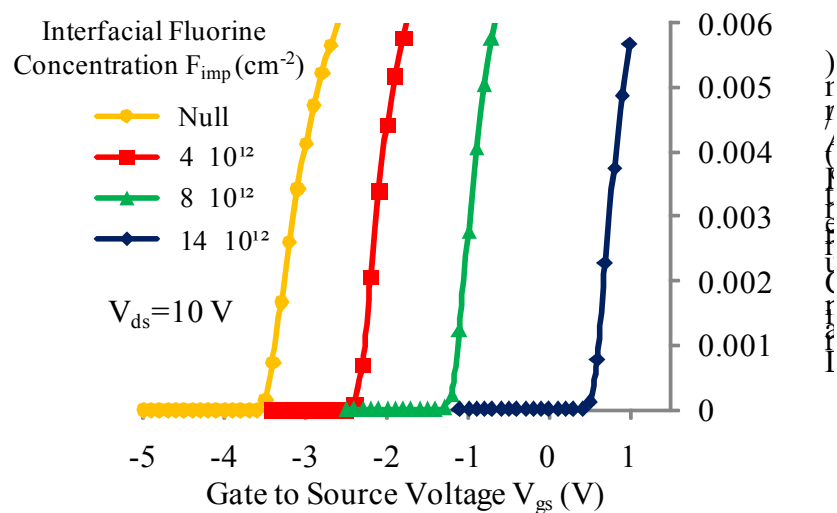
Figure 3.5 I_d (V_{gs}) transfer characteristics of the conventional normally-on HEMT and HEMTs with Fluorine implanted in AlGa 0.25 N at various concentrations
