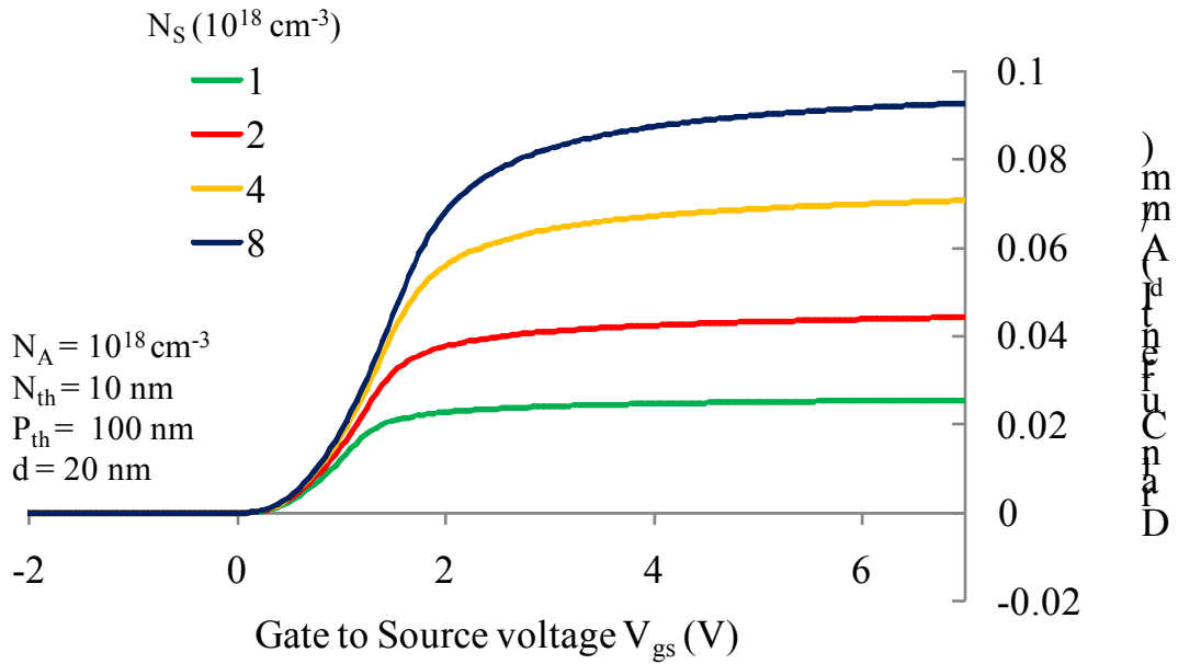
Figure 4.40 I_d(V_{gs}) transfer characteristics of structure #2 for different N_s
