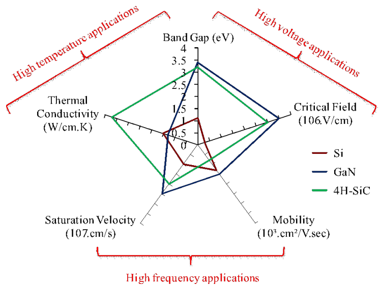
Figure 1.4 Comparison between Silicon, Gallium Nitride and Silicon Carbide based on their physical properties
