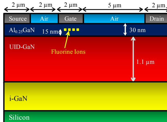
Figure 3.4 Schematic cross-section of the HEMT with Fluorine implanted in the AlGa 0.25 N layer (barrier layer)
