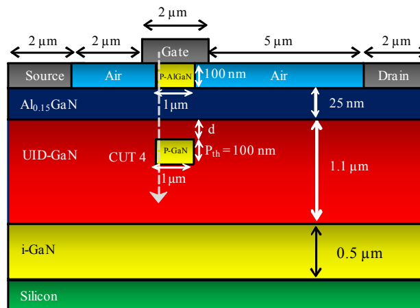
Figure 4.26 Schematic cross-section of the hybrid Gate Injection Transistor (GIT) with a buried p-GaN region
