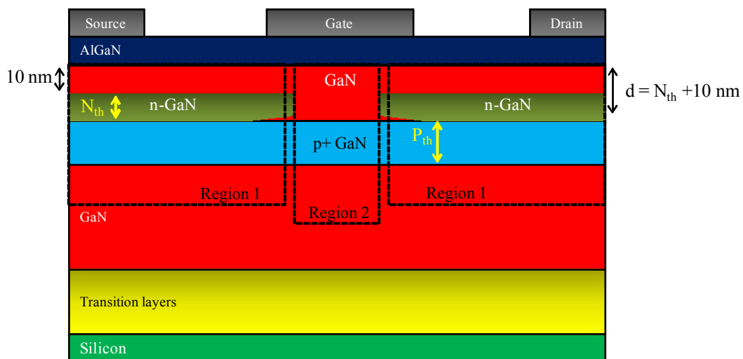
Figure 4.38 Schematic cross-section structure #2
