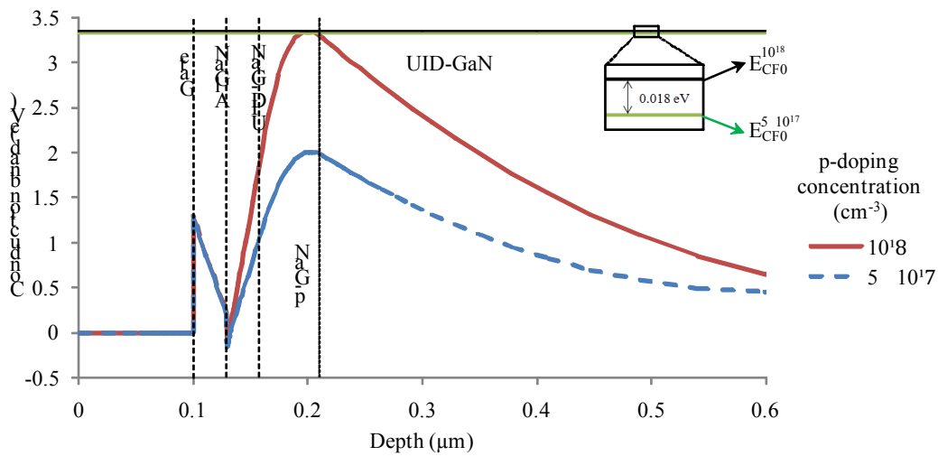
Figure 4.8 Band diagrams along CUT 2 in figure 4.2 showing the profile of the conduction band for two different doping concentrations at P_{th}=50 \text{ nm} . With higher doping concentrations, shorter thicknesses are required for E_{CF,MAX} to reach E_{CF0}
