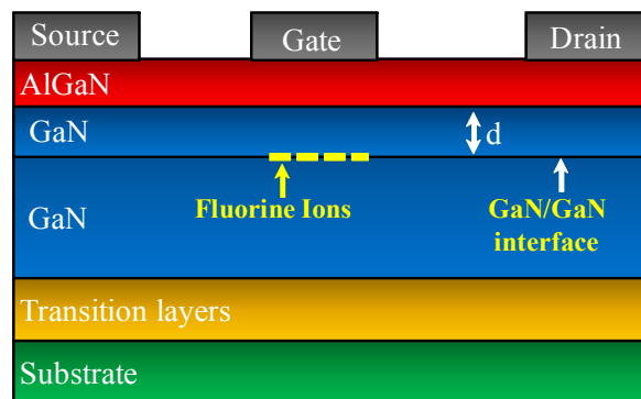
Figure 2.7 Strategy used to simulate the effect of Fluorine ions using ATLAS
