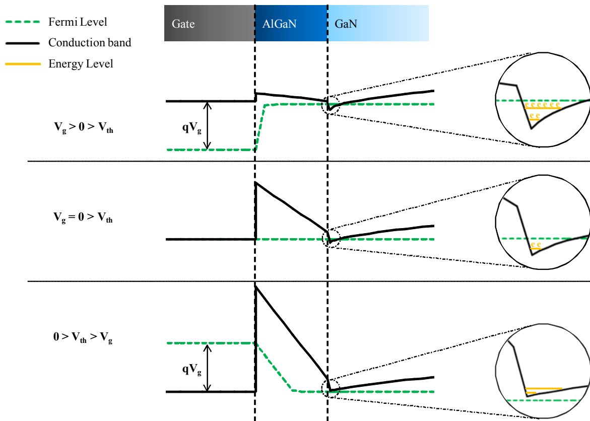
Figure 1.18 Position of the Fermi level with respect to the conduction band at various biasing conditions. The zoomed parts illustrate the status of the triangular well at the AlGaN/GaN interface to show the depletion of channel electrons (2DEG) as the gate voltage goes below the threshold voltage
