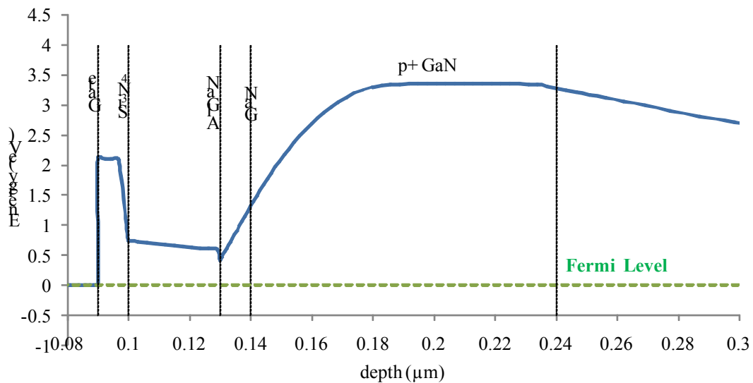
Figure 4.32 Band diagram along CUT 5 in figure 4.30 showing the elevation of the triangular well above the Fermi level, due to uplift of the conduction band in the p-region
