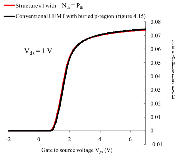
Figure 4.36 I_{ds}(V_{gs}) transfer characteristics of structure #1 at N_{th} = P_{th} and the structure shown in figure 4.15 (conventional HEMT with a buried p-region). A clear match is obtained since the two structures became identical when N_{th} = P_{th}
