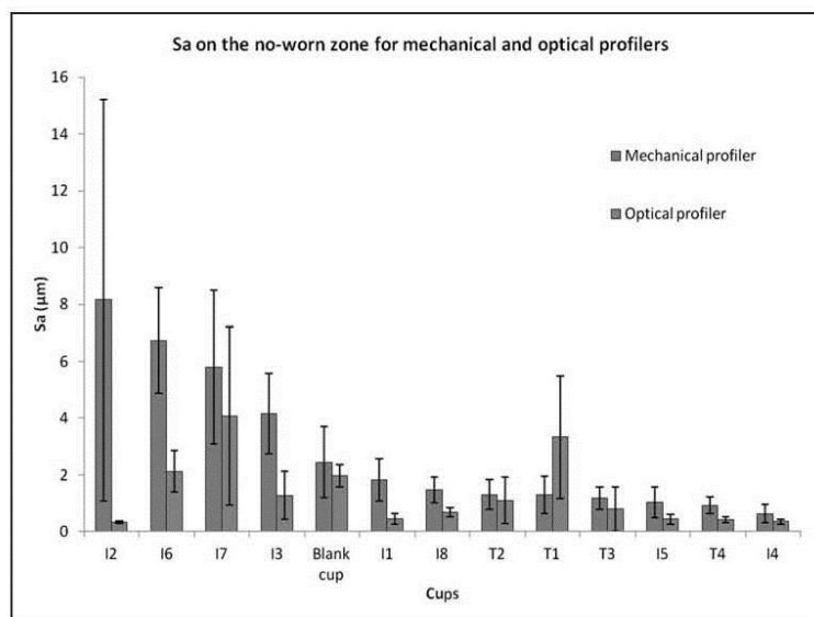
Figure 9. Sa values for every cup and both techniques on the no-worn zone ranked according to the mechanical technique.
