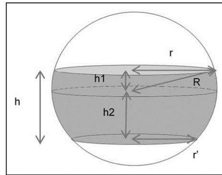
Figure 4. Spherical segment (coloured) of height h = h_1 + h_2 .
