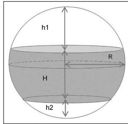
Figure 3. Spherical segment (coloured), its height is H . Two spherical caps of heights h_1 and h_2 complete the sphere of radius R . Its centre is approximated to be (0, 0, C_z) .
