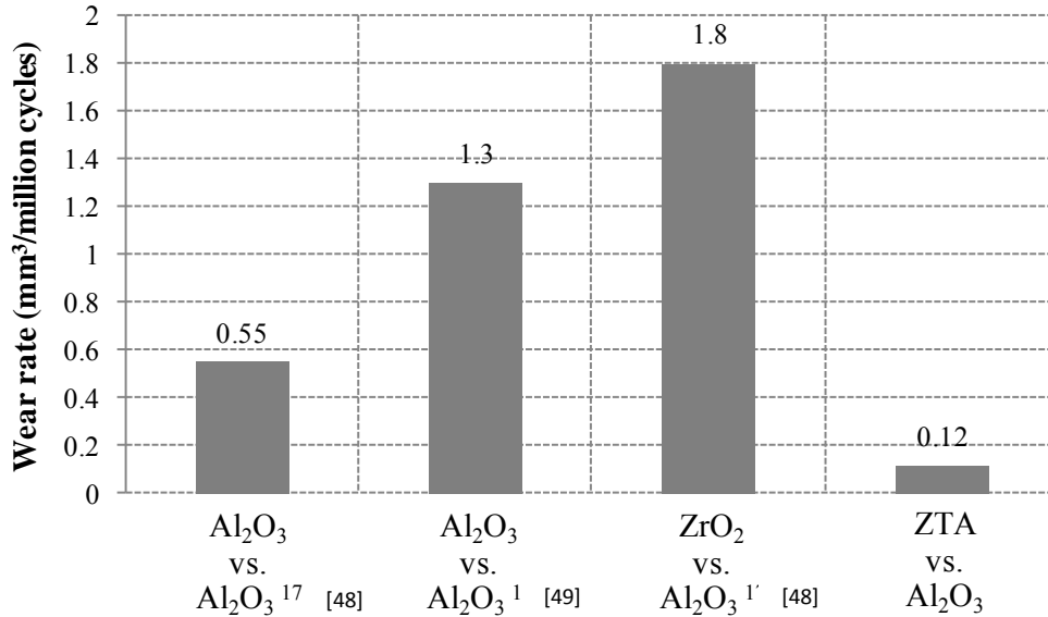
Figure 10: Wear rates of biomaterials. [48]: Steward et al., 2003, [49]: Nevelos et al., 2001.
