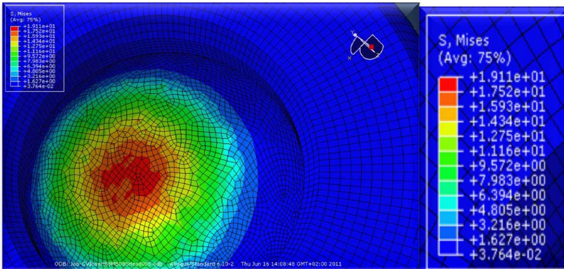
Figure 3: stresses map (von Mises stresses, MPa) inside the dual mobility cup, normal load of 2500N.
