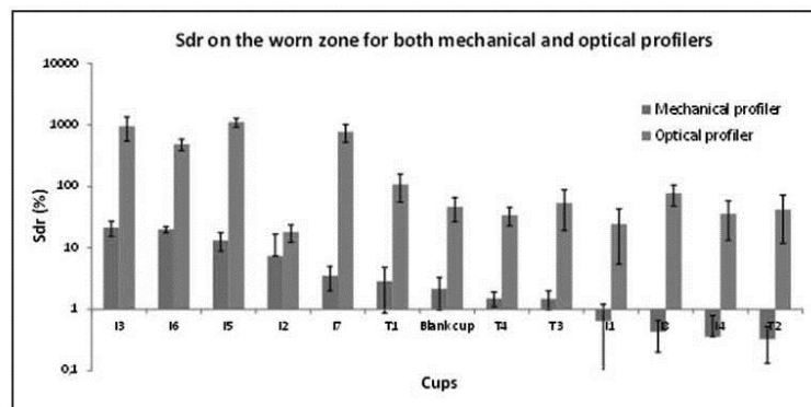
Figure 11. Sdr values for every cup and both techniques on the worn zone ranked according to the mechanical technique.
