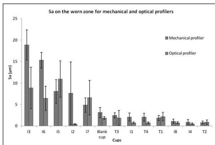
Figure 10. Sa values for every cup and both techniques on the worn zone ranked according to the mechanical technique.
