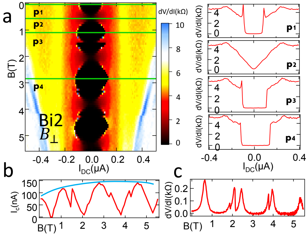
Figure 5.2.3: (a) Left panel: Color plot of the field dependence of the differential resistance of Bi 2 , with some characteristic differential resistance curves (right panel). (b) and (c) Field dependence of the critical current and zero bias differential resistance extracted from the color plot (a). Note the oscillatory behavior on the 1 Tesla field scale, and also how the maximal critical current increases with field. The blue line in (b) indicates the envelope of the critical current, increasing as the field increases.
