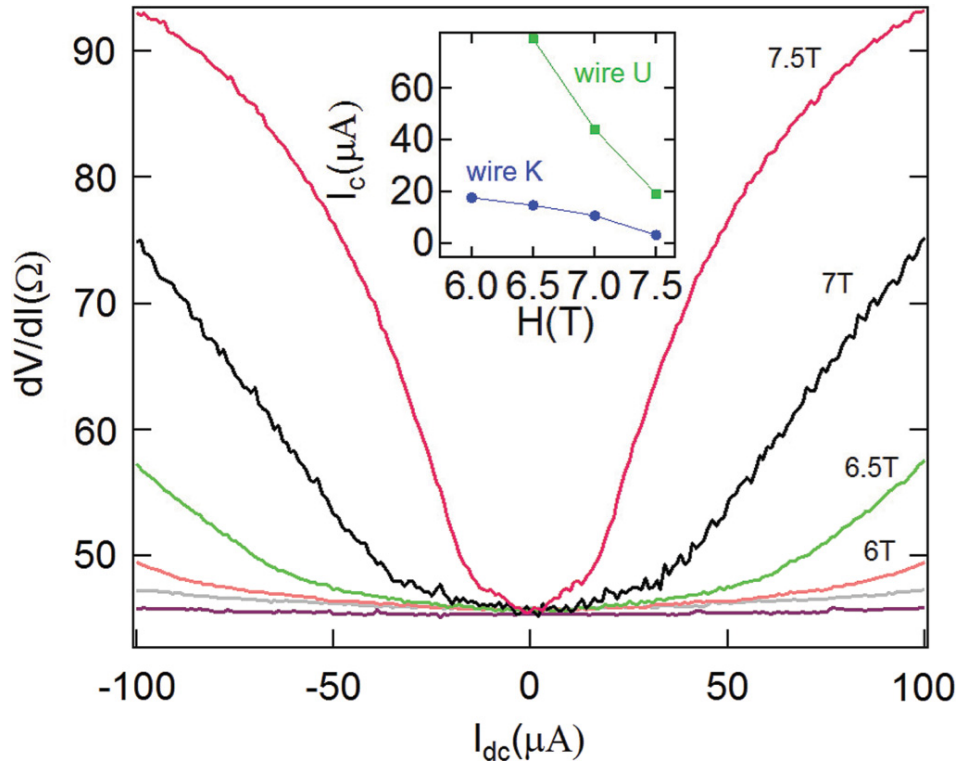
Figure A.4.1: Differential resistance of a ReW wire at different magnetic field, low temperature. (Inset) Critical current of two ReW leads.
