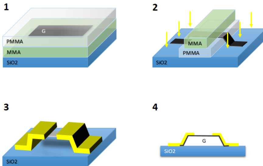
Figure A.1.4: Schematic procedures for graphene suspension with PMMA/MMA bilayer. 1) the graphene is directly exfoliated on the chip covered already by PMMA resist. Then another layer of MMA is spun on it. 2) a standard lithography procedure on top of the bilayer resist. 3) after deposition of the metal contacts, one proceed the lift-off of PMMA and MMA bilayer and finally the contacts remain and support the graphene suspension 4) side-view of this structure.
