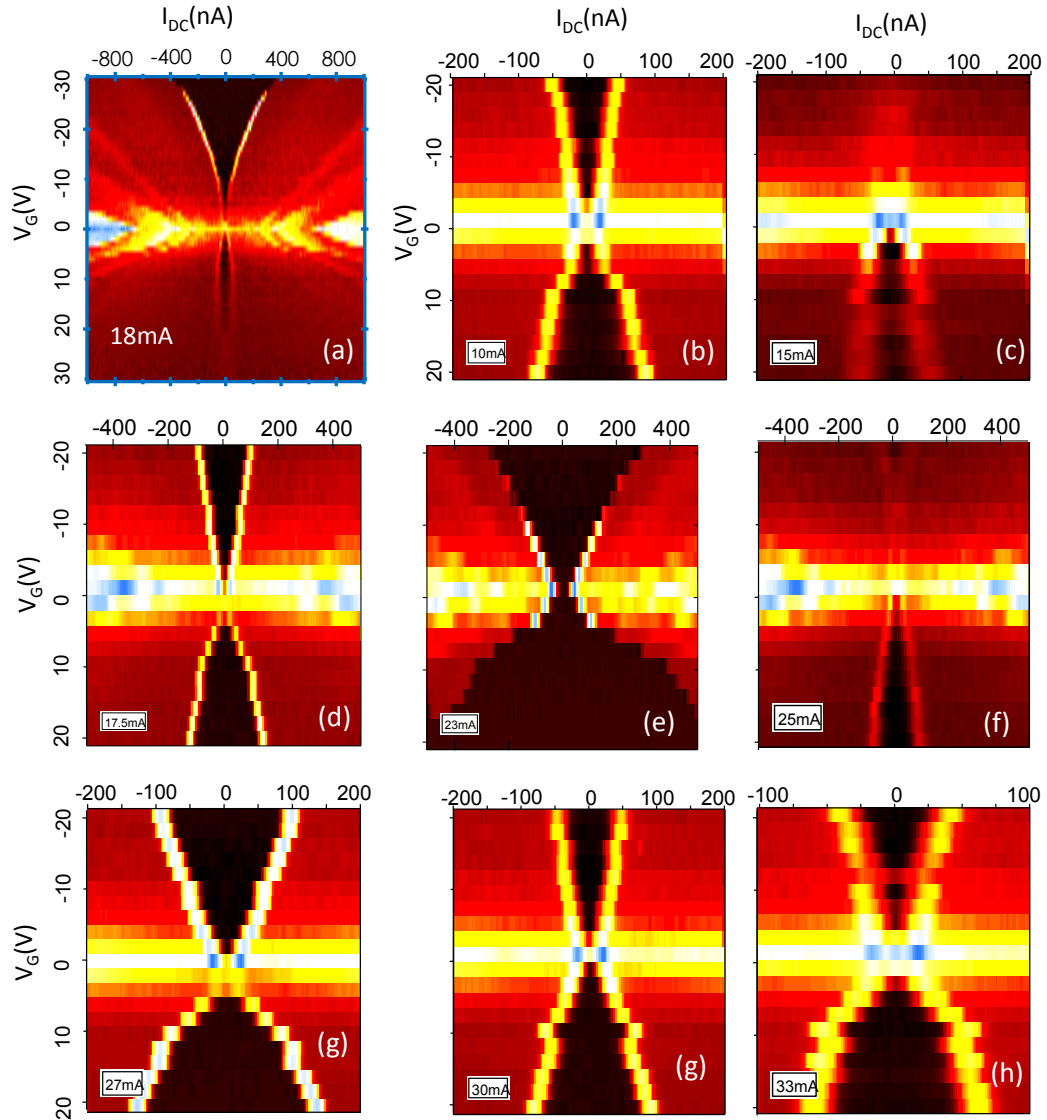
Figure 4.4.4: Gate dependent critical current of sample MC with porphyrins in different magnetic field (a) measured before increasing the field to 100G. A strong asymmetry in gate dependent critical current. (b-h) I_c(V_G) for different field.
