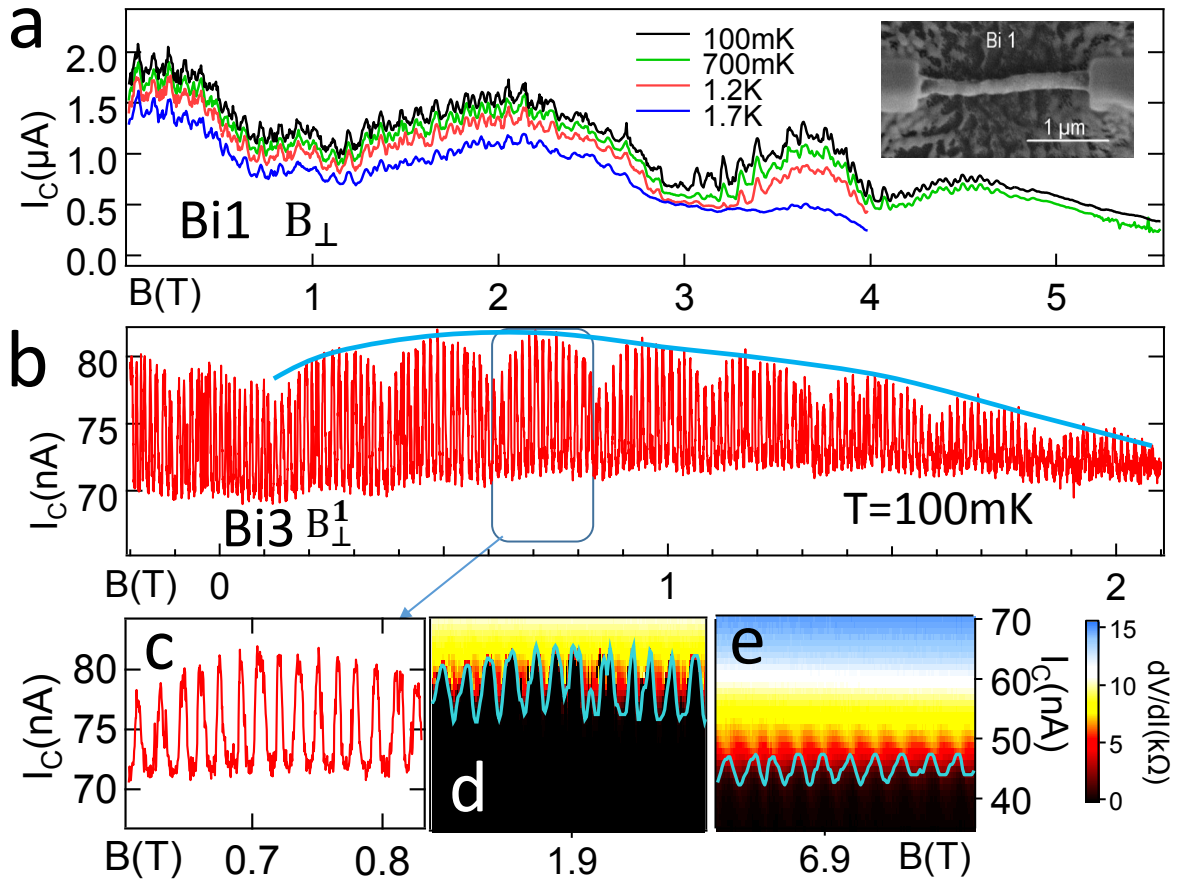
Figure 5.2.2: SQUID-like oscillations of Bi_1 and Bi_3 (a) and (b) show direct I_C measurement as function of field;(c) is the zoom figure of 2000 gauss range of (b), the blue line indicates the envelope of the whole critical current modulation; (d) and (e) are scans of dV/dI curves at different range of magnetic field, show the persistent oscillations
