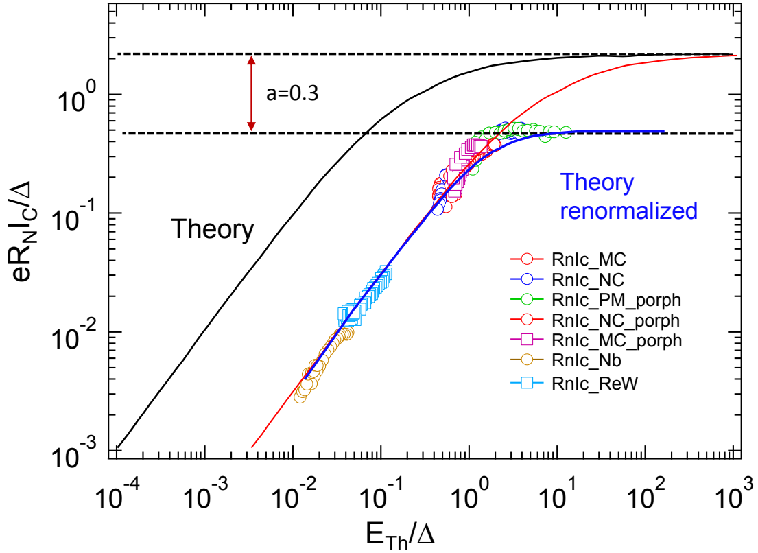
Figure 3.4.1: Normalized R_{NI_c} - E_{Th} relation for SGS samples from short junction limit to long junction limit. Same color and shape dots correspond to a same sample. All of the R_{NI_c} products are smaller than the theory curve (black) from a factor 3 to 100. Several samples present around E_{Th}/\Delta \approx 1 , it implies that these samples are in the intermediate region and should behave like short junction. The shortest sample PM, which shows flat curve at doped region, is really in short junction limit. Nb and ReW samples depend linearly on E_{Th} with the same slope (the red curve is horizontal translation of the theory curve) in the long junction limit.
