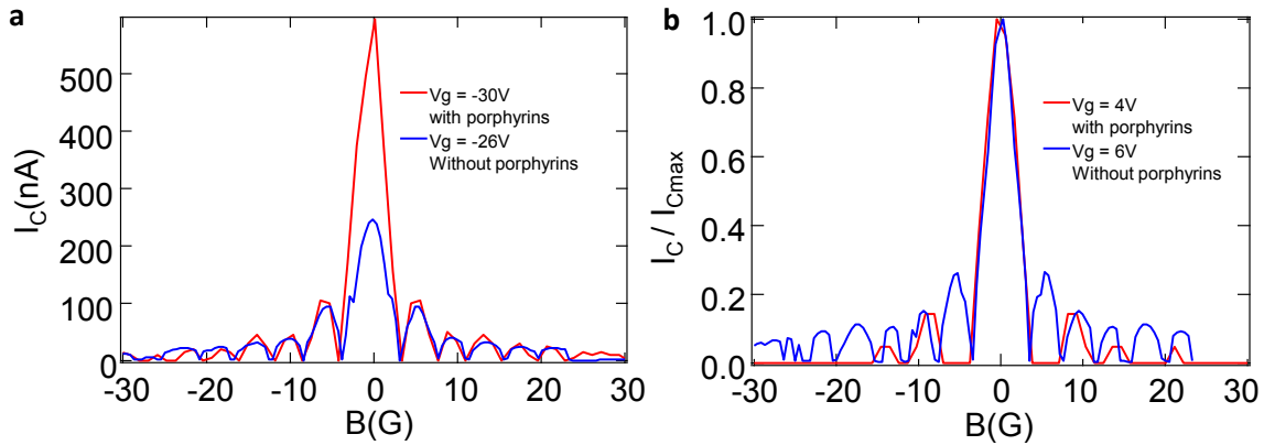
Figure 4.4.2: Fraunhofer pattern of sample MC before (blue) and after (red) grafting porphyrins at different gate voltages (a: negative values; b: positive values, normalized I_c / I_c^{max} ). All the curves' minimum is shifted to zero.
