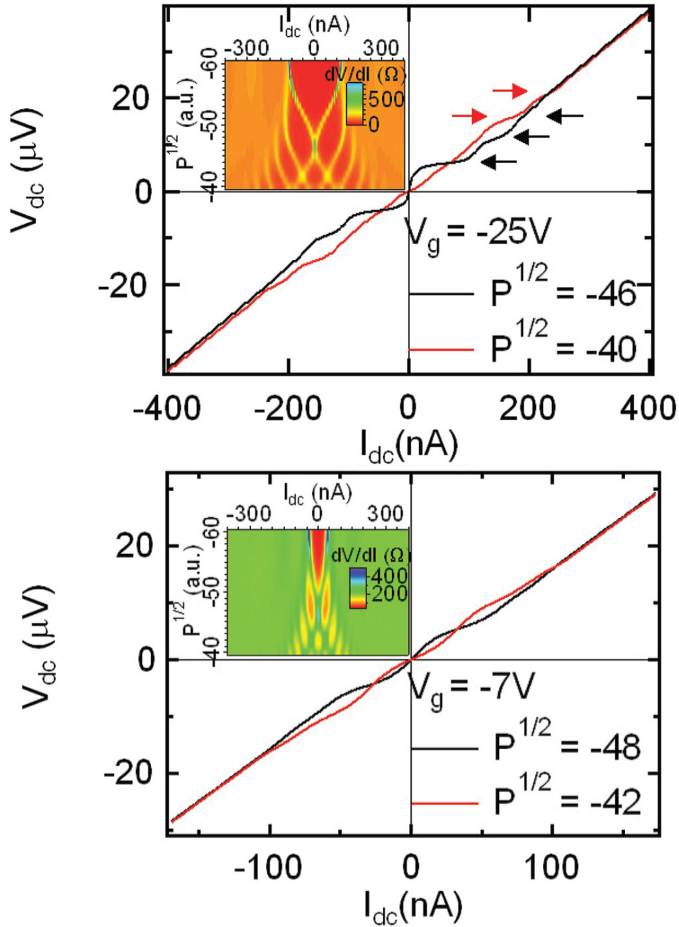
Figure 3.3.9: Effect of radio frequency irradiation on the junction with ReW electrodes.
