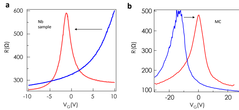
Figure 1.0.5: Gate dependence of resistance before and after the deposition of porphyrins for two samples, (a) Nb sample, (b) G92TiAl_MC. Without porphyrins (blue curves), the samples can be hole doped (a) and electron doped (b). After grafting porphyrins, in both case, the Dirac point of graphene is brought to zero, graphene becomes neutral. This implies that charge transfer occurs between graphene and porphyrins and the molecules can be donors (a) as well as acceptors (b) of electrons.
