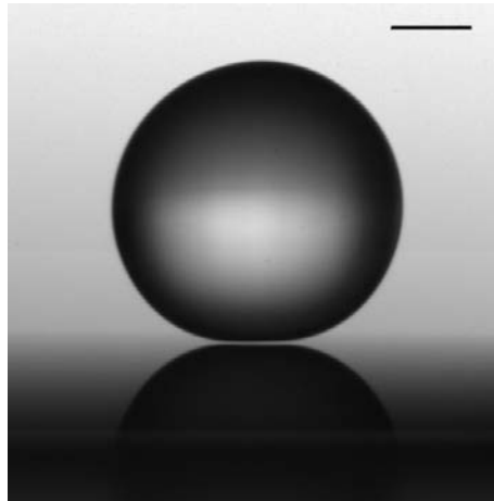
Figure I.5 – Side view of a water droplet on a hot substrate (400°C). The gap between the drop and the substrate (visible because of the back light passing through it) has a typical height h \sim 100 \mu\text{m} . The bar shows 1 mm.
