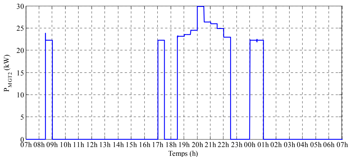
Fig.4.79. P_{MGT\_2}
