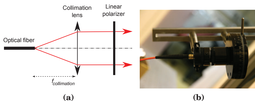
Figure 3.2: Illumination system. (a) Schematic view of the illumination system. A lens of focal length f_{\text{collimation}} collimates the output of an optical fiber. The parallel rays then pass through a linear polarizer to obtain TE or TM polarized light. (b) Picture of the illumination system.
