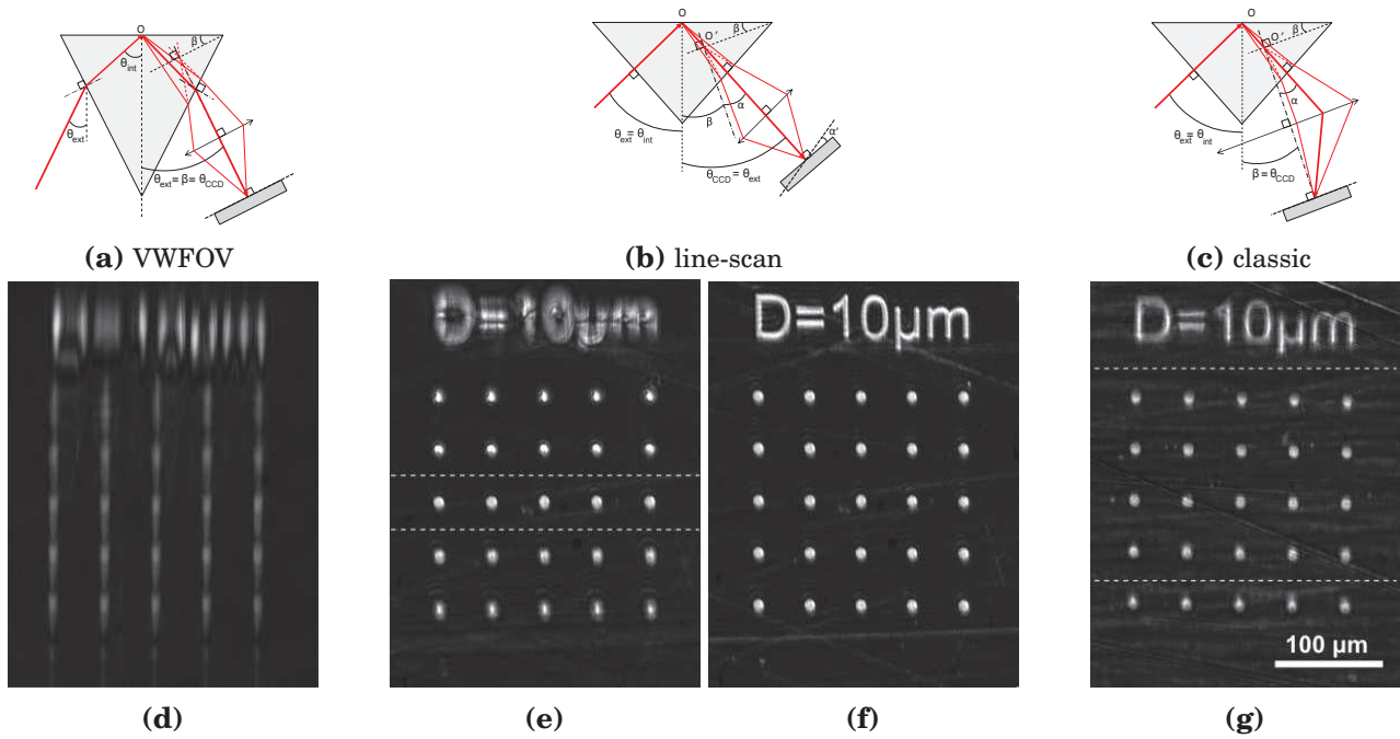
Figure 4.1: Small FOV comparison between the three optimized configurations on SF11 prisms ( \lambda = 632 \text{ nm} , water, d \approx 5 \text{ mm} ). (a & d) VWFOV optimized prism (SF11, OL: \times 20 , TL: 200 mm). (b, e & f) Resolution optimized prism in line-scan imaging mode (100 lines, SF11, OL: \times 20 , TL: 200 mm). Figure e is an example of a single intermediate image. (c & g) Resolution optimized prism in classic imaging mode (SF11, OL: \times 50 , TL: 65 mm).
