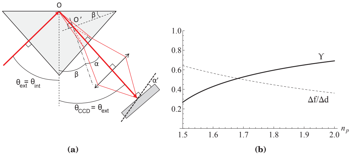
Figure 2.8: Line-scan imaging mode with resolution optimized prisms. (a) Optical scheme with a N-SF66 prism, A_p = 83^\circ , \theta_{int} = 48.5^\circ . (b) Anamorphose and focus adjustment in line-scan imaging mode.
