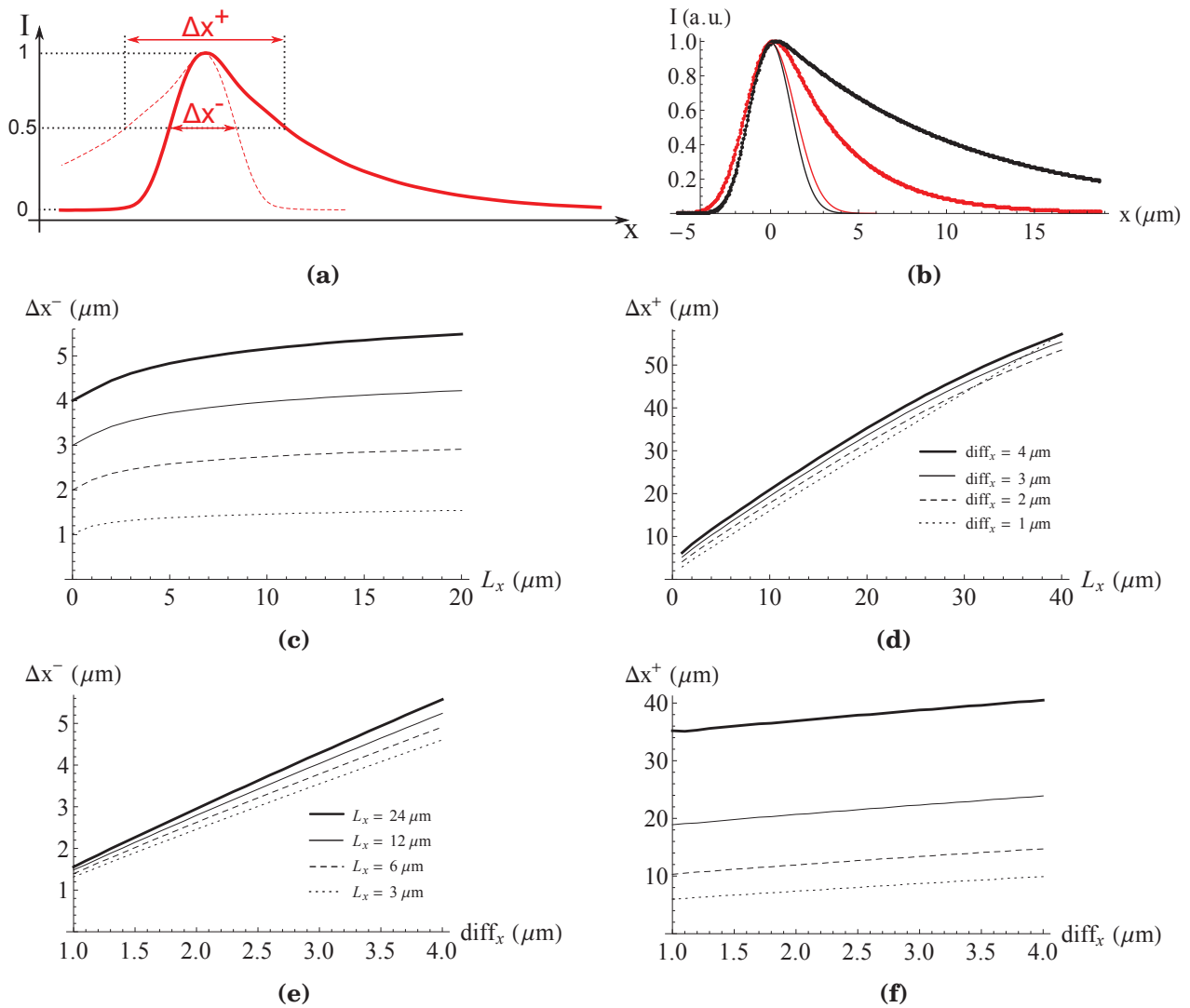
Figure A.18: \Delta x^- and \Delta x^+ as a function of L_x and diff_x . (a) Illustration of \Delta x^- and \Delta x^+ on the PSF. (b) Example of determination of \Delta x^- by a Gaussian fit of the left part of the theoretical PSF parallel to the SP at \lambda = 632 (red) and 721 nm (black). The value of diff_x and L_x are the ones from the free fits of Section 4.2.3 . (c) \Delta x^- as a function of L_x for different diff_x . (d) \Delta x^+ as a function of L_x for different diff_x . (e) \Delta x^- as a function of diff_x for different L_x . (f) \Delta x^+ as a function of diff_x for different L_x .
