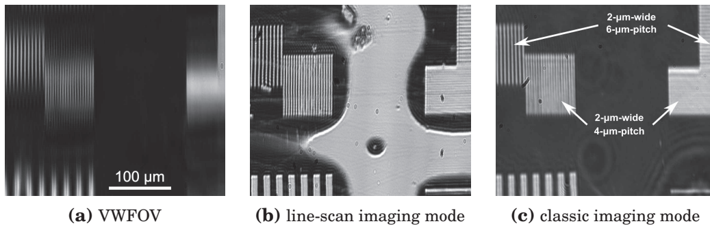
Figure 4.2: X and Y axis spatial resolution for VWFOV and resolution optimized prisms (SP propagate downward, \lambda = 632 \text{ nm} , water, d \approx 5 \text{ mm} ). (a) VWFOV optimized prism (SF11, OL: \times 20 , TL: 200 mm). (b) Resolution optimized prism in line-scan imaging mode (125 lines). A air bubble is trapped between the PDMS and the prism (SF11, OL: \times 20 , TL: 200 mm). (c) Resolution optimized prism in classic imaging mode (N-SF66, OL: \times 50 , TL: 65 mm).
