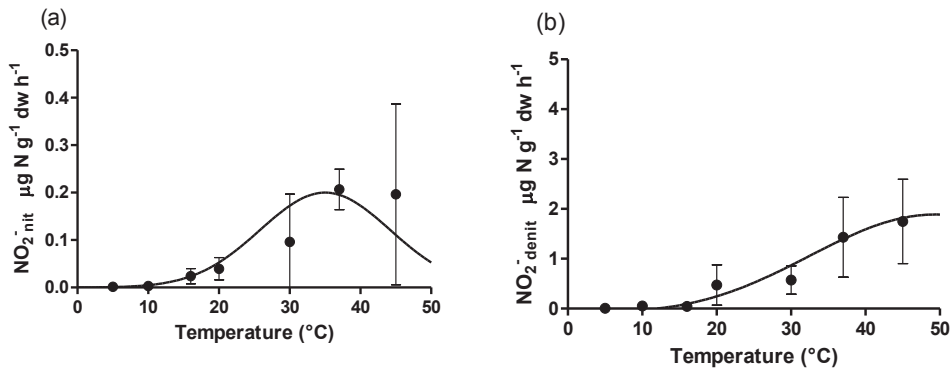
Figure 4-2. Nitrite net productions from ammonium oxidation during nitrification (a), i.e., \text{n}_\text{T-m}_\text{T} , and from nitrate reduction during denitrification (b), i.e., \text{a}_\text{T-b}_\text{T} , with means and SD. The curve corresponds to the best fit of a sigmoid function based on all data observed, with R^2 = 0.3 for nitrification (a) and R^2=0.5 for denitrification (b). Scale for denitrification is ten times greater than for nitrification
