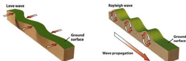
Figure 2.2 Surface waves: Rayleigh and Love.
