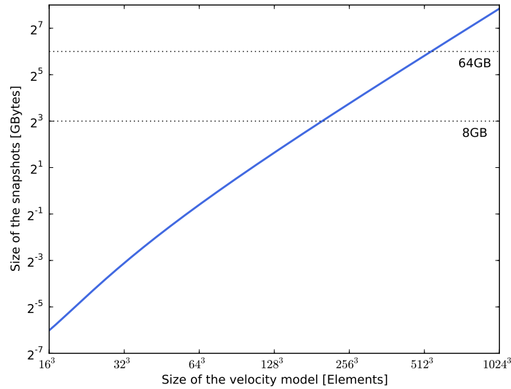
Figure 6.8 Size of snapshots as a function of the velocity model size. We give memory size on Sandy Bridge (64GB) and on MIC (8GB) as upper bounds on a KNC node.
