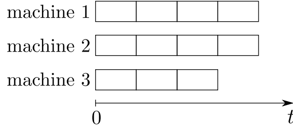
Figure 20: Static scheduling on 3 identical machines
