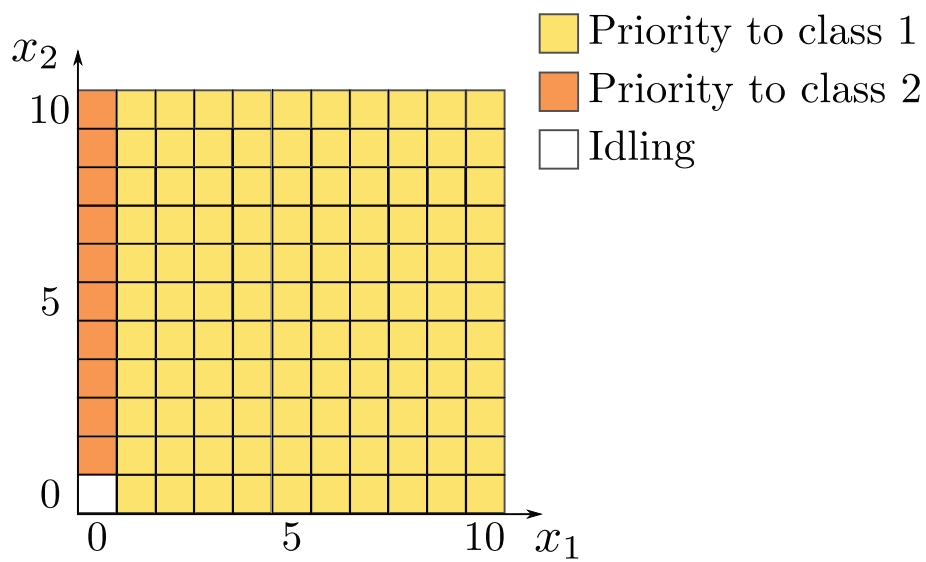
Figure 27: Example of non idling policy
