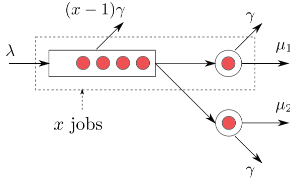
Figure 23: Problem with a single class of jobs and with two machines of different exponential rates
