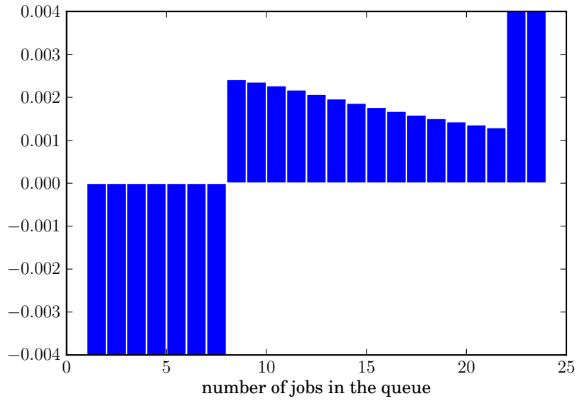
Figure 25: Value of \Delta_{e_x, -e_x + e_u} v(x+1, 0) for the instance M = 25 , \mu_1 = 3 , \mu_2 = 0.5 , \lambda = 2 and \gamma = 1
