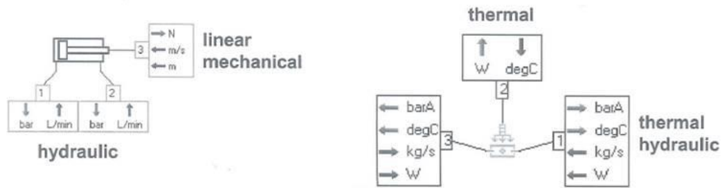
Figure 6 Multiple Regrouped Variables Representation in AMESim Tool
