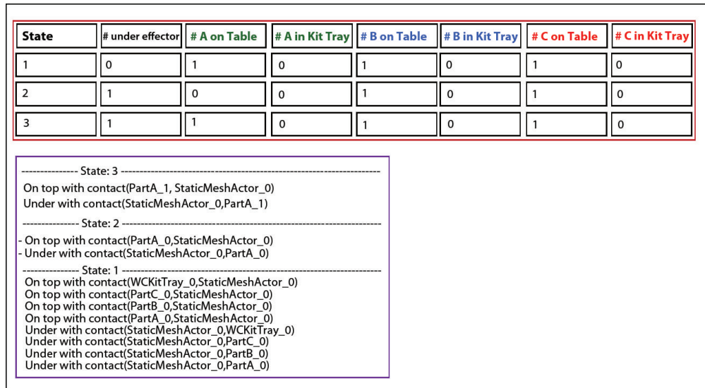
Figure 52: Results of State Recognition Algorithms
