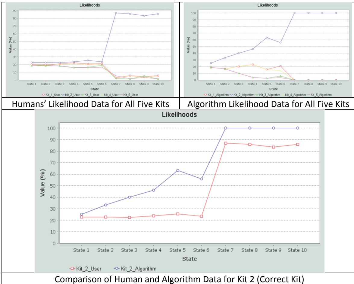
Figure 68: Human/Algorithm Comparison Data for Kit 2 Plan 5
