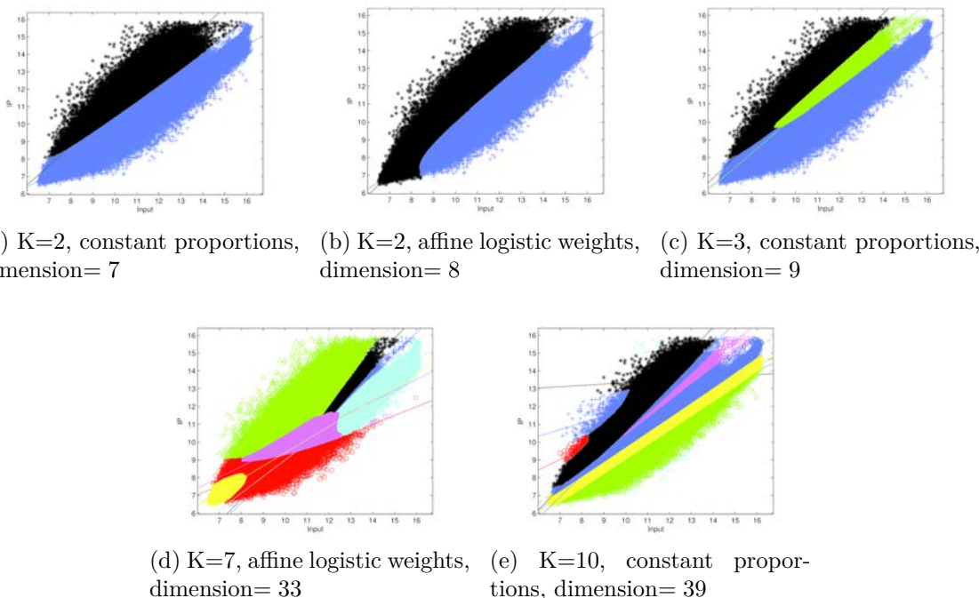
Figure 2.10 – Clustering of ChIP-chip data set into K classes.
