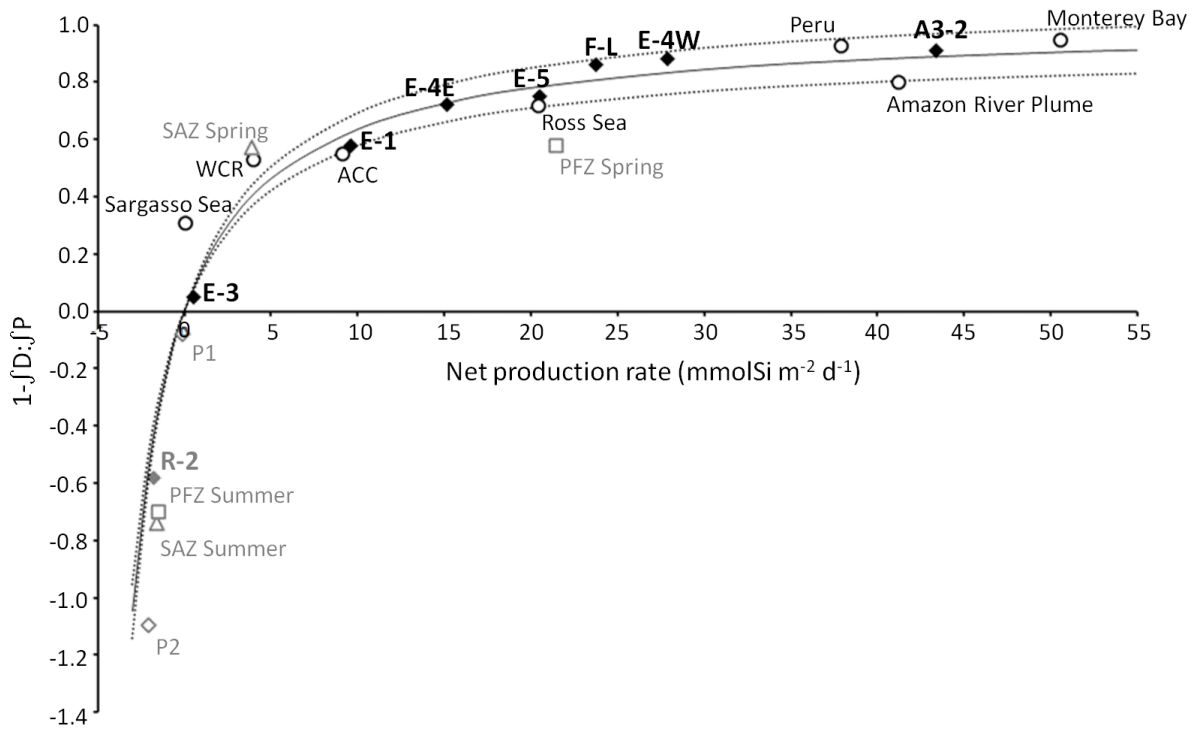
Figure 1.7. Fraction of biogenic silica production supported by new silicic acid ( 1-fD:jP ) as a function of the integrated net silica production rate ( jP_{net} ) during KEOPS-2 (filled black diamonds) compared with different regions of the global ocean (Open circles; Brezinski et al., 2003 and references therein; and open diamonds; Fripiat et al., 2011b). Triangles and squares show the mean values for different growth seasons for SAZ and PFZ, respectively (Fripiat et al., 2011b). The plain line is a rectangular hyperbola to fit all data points (grey symbols were excluded from the model since they represent either negative 1-fD:jP value which are not allowed by the model, or average while all other symbols refer to single stations). The equation of the curve is 1-fD:jP = 1.01 \times jP_{net} / (5.89 + jP_{net}) . Dotted lines correspond to \pm 1 sd of the 1-fD:jP_{max} .
