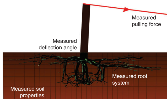
FIG. 1. Anchorage model with root system architecture and soil properties measured for tree-pulling simulations. Model outputs are the response curve of turning moment versus the deflection angle at the stem base and the total energy supplied by the pulling force. Deflection angle is defined as the angle between the vertical and the stem.
