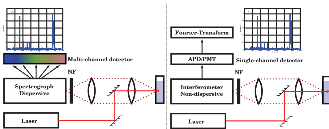
Figure 2.7: Dispersive and non-dispersive configurations of Raman spectrometer devices.
