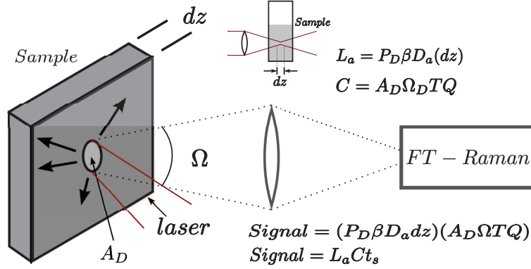
Figure A.1: Diagram of the variables involved in the generation and detection of Raman scattering light in a 180^\circ back-scattering geometry. Figure reproduced from [109, p. 36].
