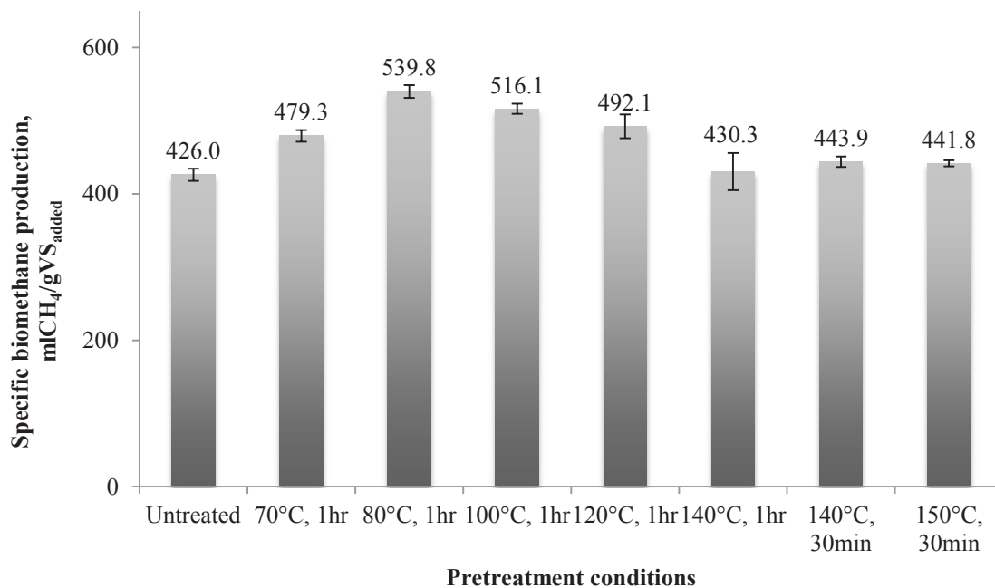
Figure 3.2: Effect of thermal pretreatment on the specific biomethane production during the initial 20 days of the BMP test
