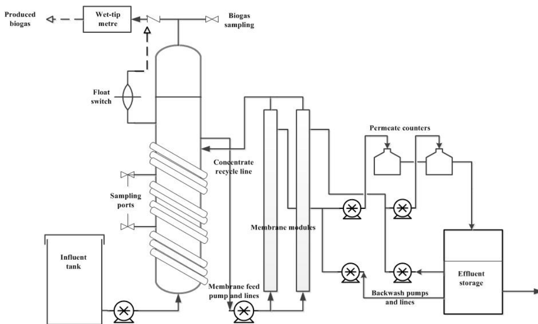
Figure 8.1: Schematic diagram of AnMBR
