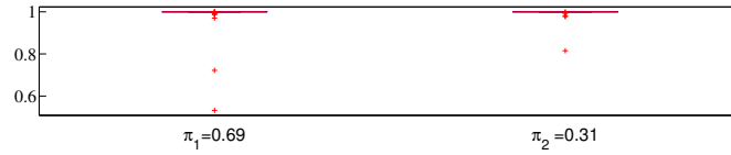
Figure 5.9: Assignment boxplots per cluster
