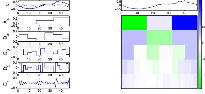
Figure 5.2: Projection of a load consumption for one day into Haar basis, level 4. By construction, we get s = A_4 + D_4 + D_3 + D_2 + D_1 . On the left side, the signal is considered with reconstruction of dataset, the dotted being preprocessing 1 and the dotted-dashed being the preprocessing 2
