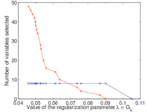
Figure 1.2: For one simulation, zoom in on number of false relevant (in red color) and true relevant (in blue color) variables generated by the Lasso, by varying the regularization parameter \lambda around the interesting values
