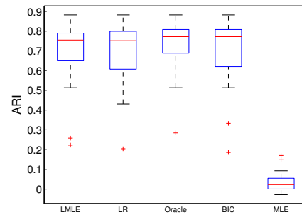
Figure 1.10: Boxplots of the ARI over the 20 simulations, for the Lasso-MLE procedure (LMLE), the Lasso-Rank procedure (LR), the oracle (Oracle), the BIC estimator (BIC) and the MLE (MLE) for the model 4
