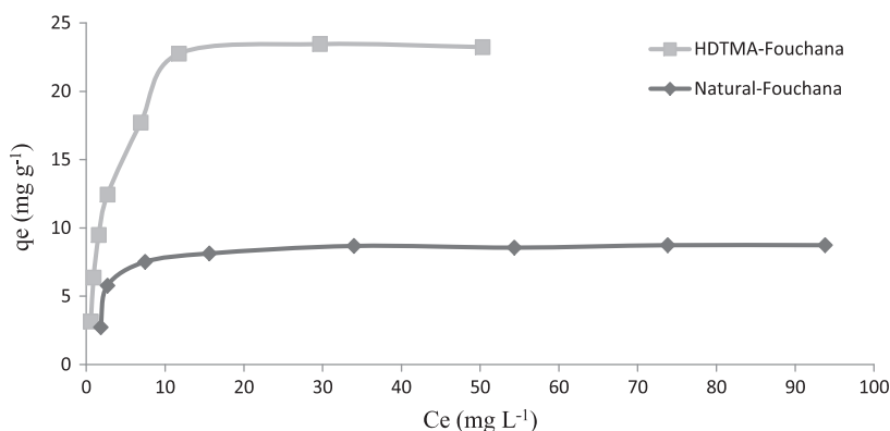
Fig. 5. Effect of initial RR120 dye concentration on the adsorption onto Fouchana and HDTMA-Fouchana clays (pH = 6, T = 25^{\circ}\text{C} ).
