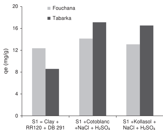
Fig. 6. Effect of the dyeing additives Cotoblanc and Kollasol at high ionic strength (NaCl 1 M) and low pH (5.5 to 6.5), on the amount of mixed dyes (RR 120 and DB 291) adsorbed onto the Fouchana and Tabarka clays at ambient temperature.
