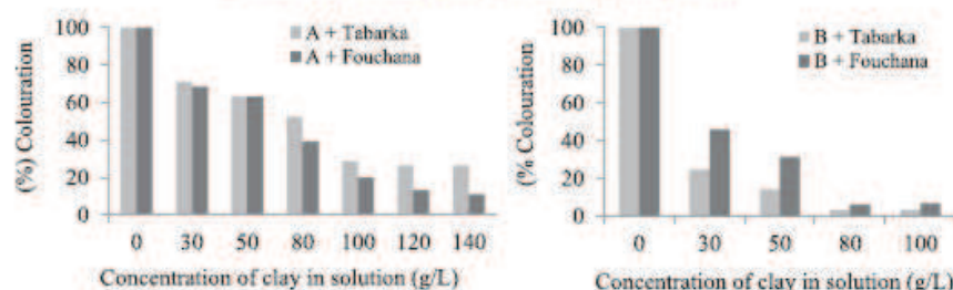
Fig. 2. Effect of Fouchana and Tabarka clay concentrations on the decoloration of real effluents A (a) and B (b).
