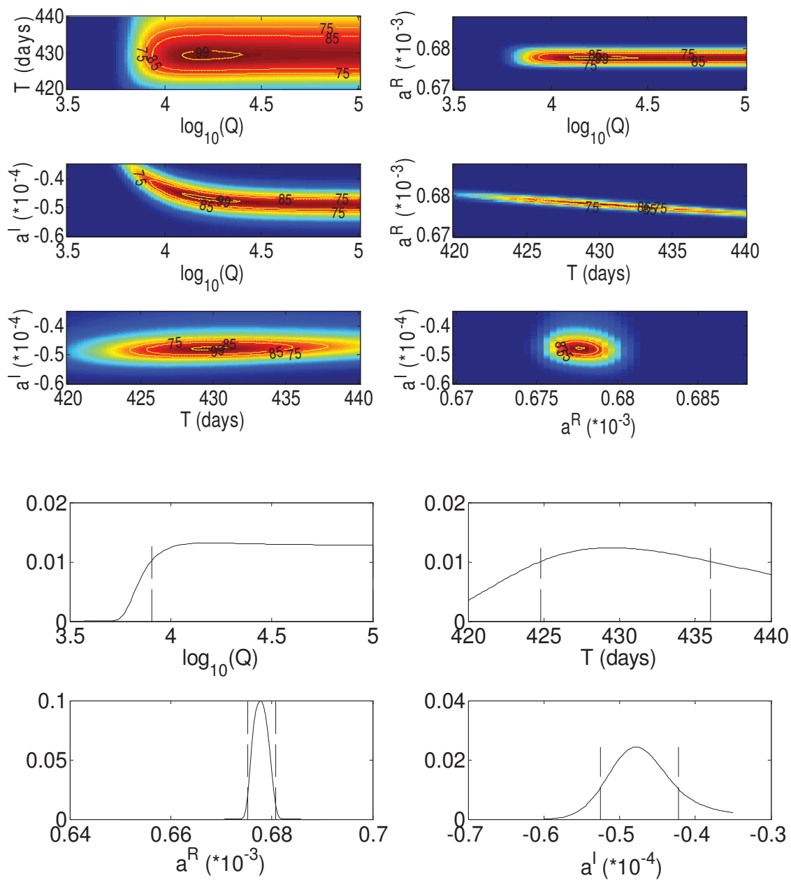
Fig. 6.11: Joint and marginal probability density functions for the FCN parameters ( a_r, a_i, T and x ) estimated from 18 years of SG C026 data using the Bayesian method. Vertical dotted lines indicate the 90% confidence intervals.
