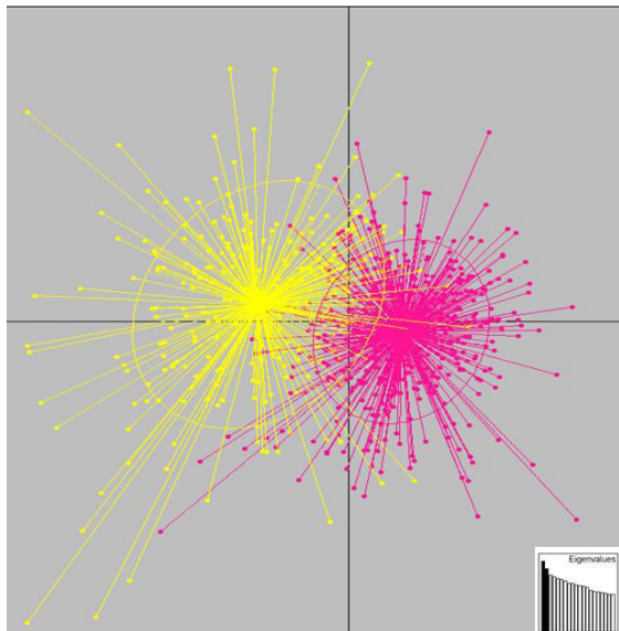
Figure 3. Principal Component Analysis Scatter plot, each colour representing a genetic cluster obtained by Structure (assuming K=2 genetic clusters), the bar graph displays the variance explained by the 2 discriminant eigenvalues used for plotting.
