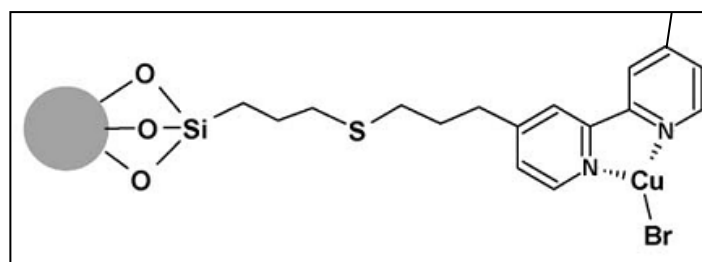
Figure 1.23: Complexe CuBr/ bipyridine.
