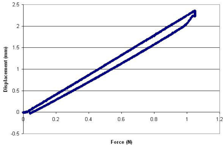
Figure 2.13: Example of 4-point bending force vs. vertical displacement data file.
