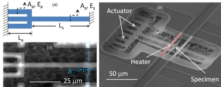
Figure 1.5: (a) Figure showing the single layer \text{SiN} three-strip actuator, (b) Scanning electron micrograph of a specimen, (c) Strain is measured post-experiment fracture of the specimen. Adapted from Alam et al. (2015) .
