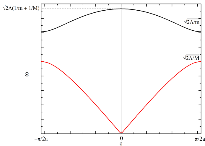
Figure 1.7: Dispersion relation for linear diatomic chain.
