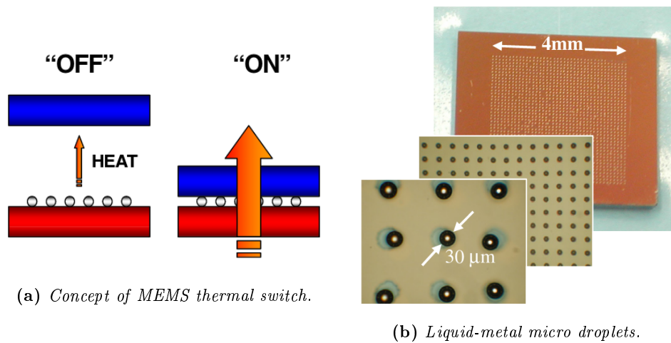
Figure 1.4: A MEMS thermal switch schematic and real-life counterpart. Adapted from Cho et al. (2008)
