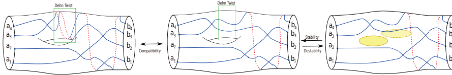
Figure 1.6: Braids in a thickened surface.
