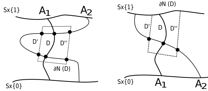
Figure 4.2: A non-horizontal circle and a non-vertical arc in A_1 .
