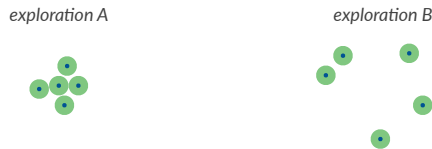
Figure 1.10: Threshold coverage is insensitive to effect spread over the threshold. The two explorations have the same threshold coverage.
