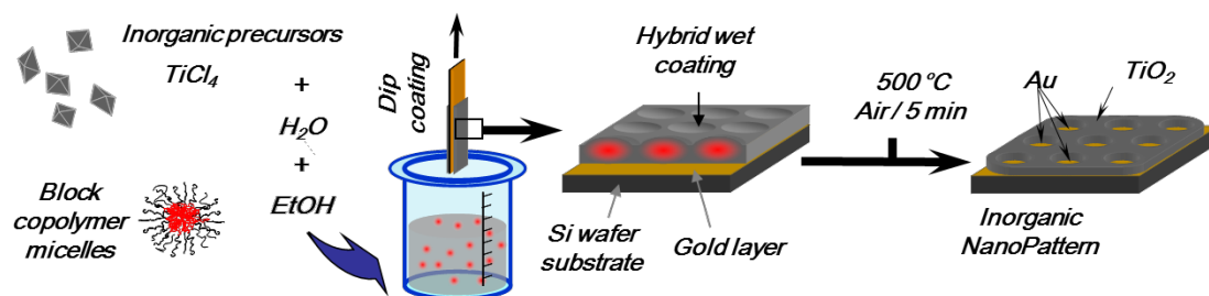
Scheme 1: Fabrication of the nanoporous \text{TiO}_2 layer (steps 2 and 3).
