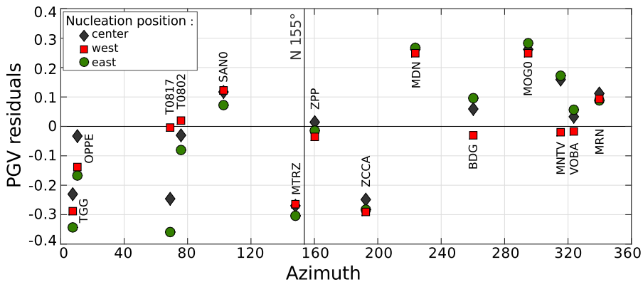
FIGURE 4.9 – Comparison of PGV residuals between the mean values of simulations, for different nucleation positions, with the data. Residuals are computed as the difference between the \log(\text{PGV}) of simulations with the \log(\text{PGV}) from data.
