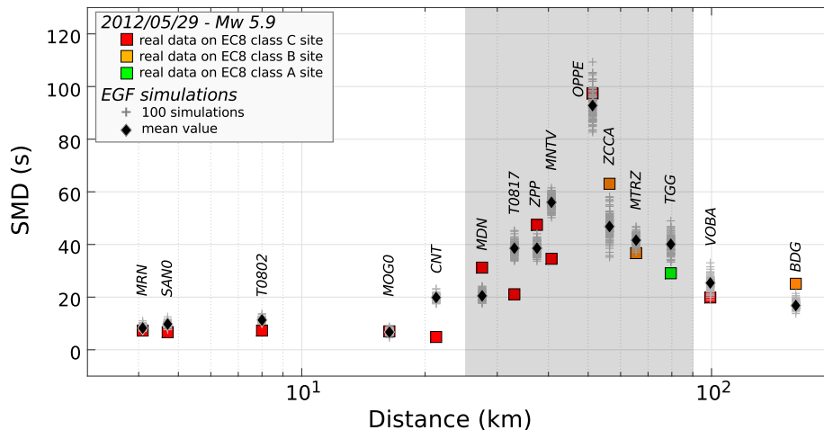
FIGURE 4.5 – Comparison between observed and simulated Strong Motion Duration (SMD defined as the time between 5% and 95% of the Arias Intensity (Trifunac and Brady, 1975)). Arias intensity is computed on the acceleration time series filtered between 0.2 and 35 Hz.
