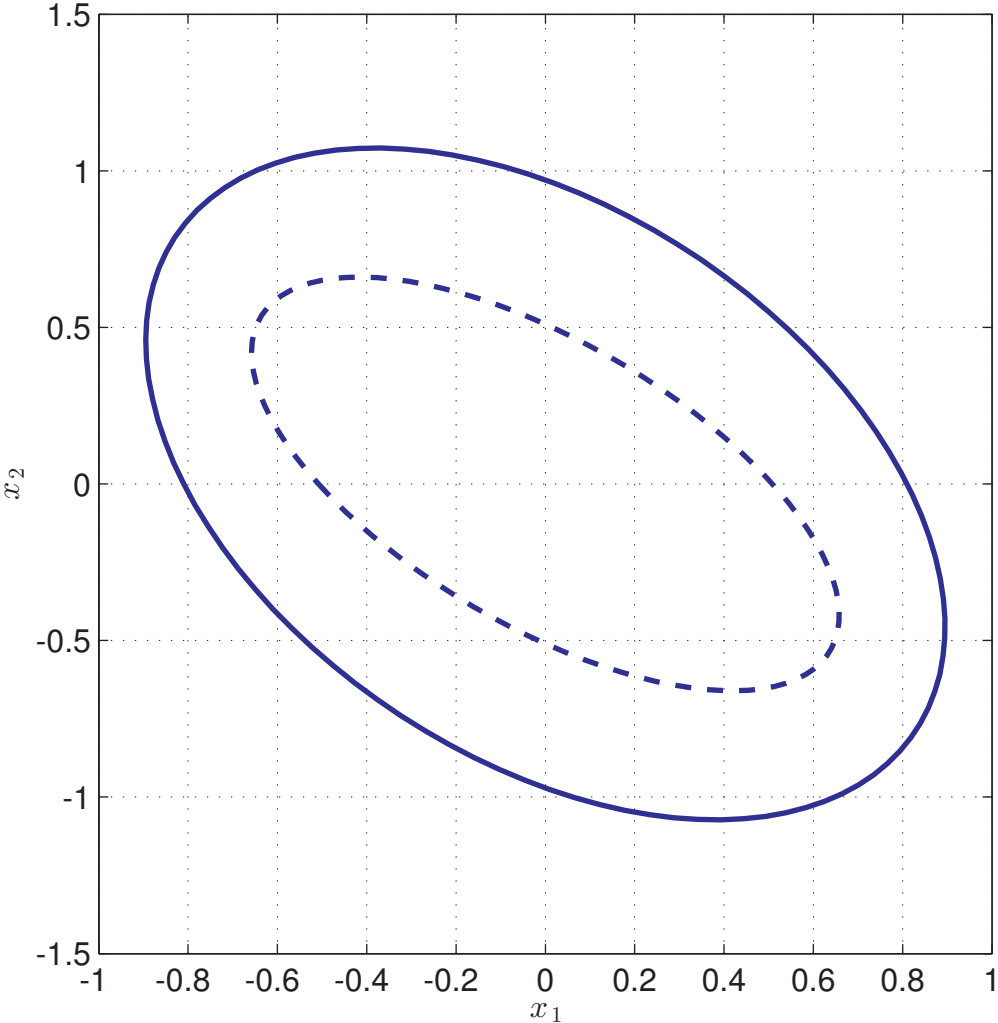
Figure 2.4: The two sets \mathcal{A} resulting from the solution to the controller design problem. \mathcal{E}(W^{-1}) solid, \mathcal{E}(F^{-T} J F^{-1}) dashed.
