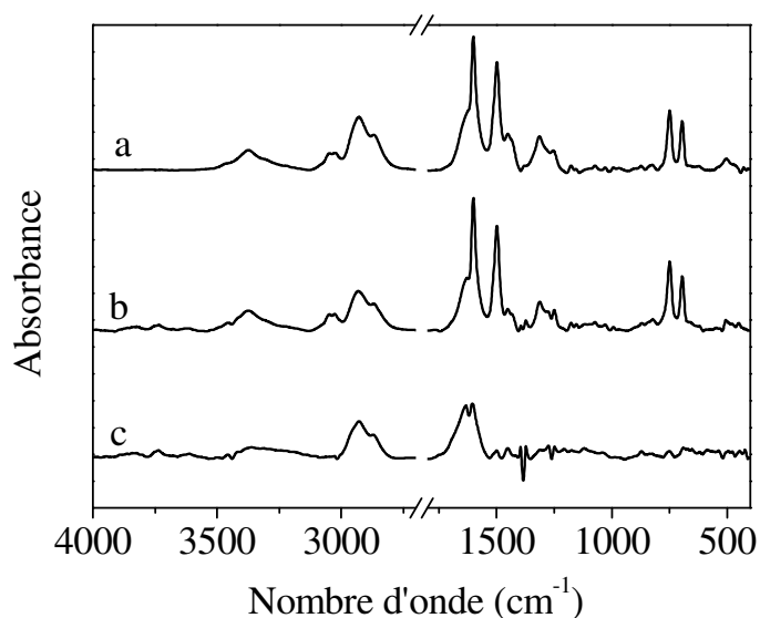
Figure 3-5. Spectres FTIR des couches obtenues : a) T_{ANi}=40^{\circ}C , T_{sub}=20^{\circ}C ; b) T_{ANi}=40^{\circ}C , T_{sub}=10^{\circ}C ; c) T_{ANi}=20^{\circ}C , T_{sub}=10^{\circ}C .
