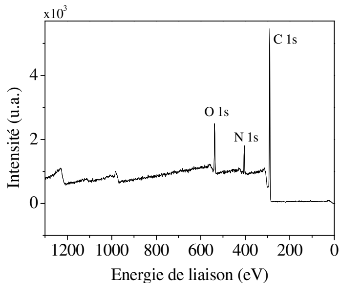
Figure 3-8. Spectre XPS large de PANi. P=60 W, T ANi =40°C, T sub =10°C, t=10 min.
