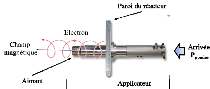
Figure 2-2. Applicateur ECR
