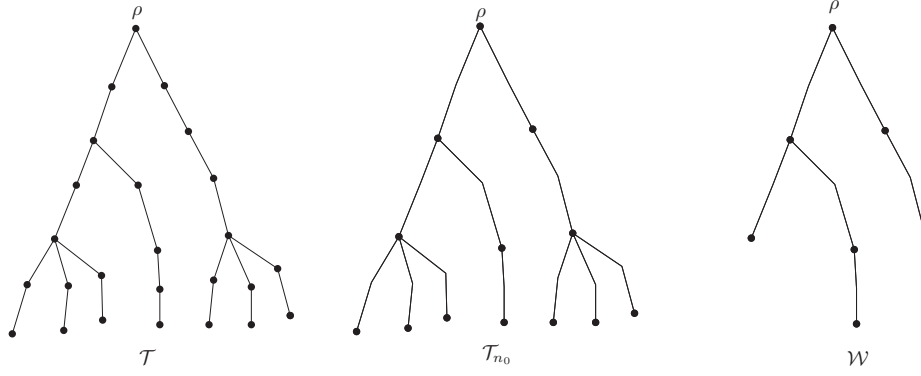
Figure 4.3: An example in the case K_0 = n_0 = 2 .
