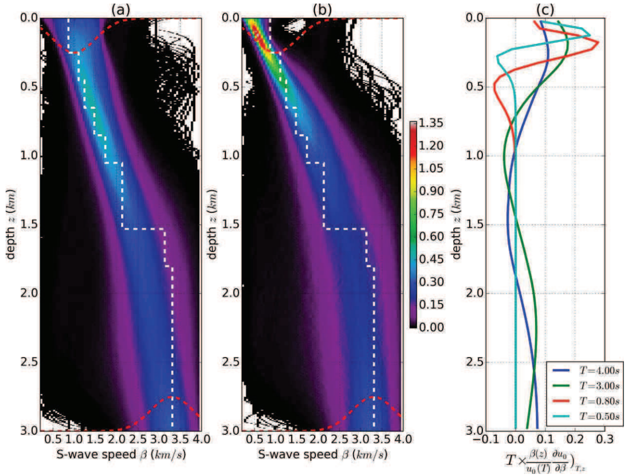
Figure III.33 : Shear-wave velocity profile obtained between the two arrays ARIT and AKUL using the group velocity dispersion curve of the fundamental mode of Rayleigh wave shown on figure III.32. (a) : Inversion of the long period part of the dispersion curve (0.8s to 5s) determined without array processing (figure III.32, right side of the white dashed line). The color scale corresponds to the a posteriori probability density function over the model space evaluated by MCMC. The white dashed lines represent the 1 dimensional model of Soultz-sous-Forêts (see Beauce et al., 1992 ; Charl  ty et al., 2006 ; Cal   et al., 2013). The red dashed Gaussian functions correspond to the prior constraints imposed to the shear wave velocity at the surface and at 3km depth. (b) Inversion of the combined dispersion curve over the entire range of period 0.2 to 5s obtained with ( <0.8s ) and without ( >0.8s ) array processing (figure III.32, full dispersion curve). (c) Depth sensitivity kernels of the group velocity dispersion curve (noted u_0(T) ) with respect to shear wave velocity \beta at four periods. The amplitudes of the kernels are multiplied by the period ( T ) to balance the amplitude decay at long period.
