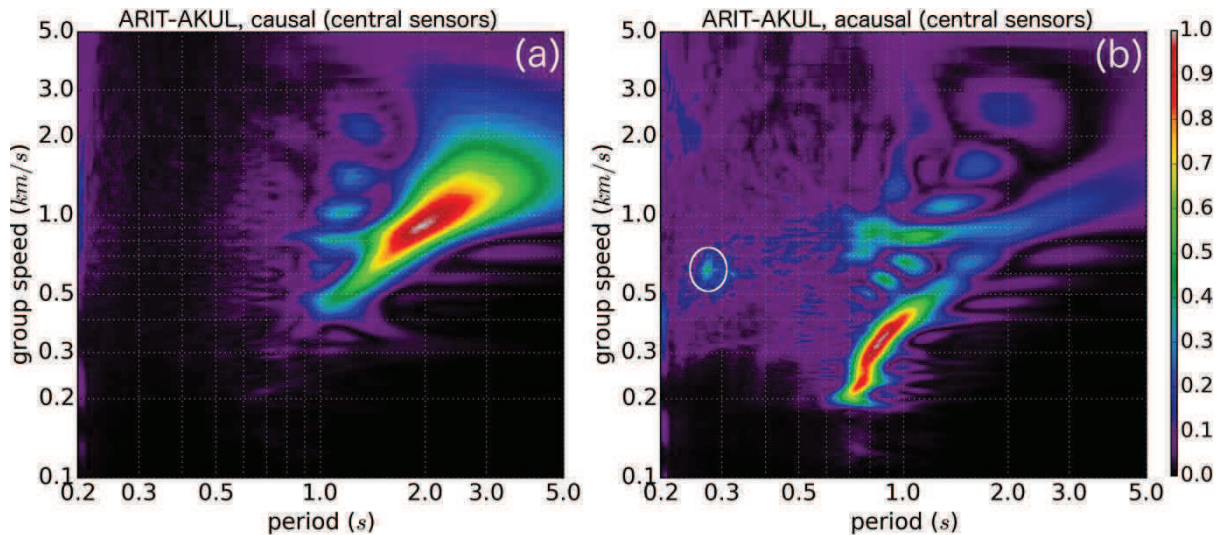
Figure III.29 : Group speed dispersion obtained by frequency time analysis of the cross-correlation function between the central sensors of the arrays ARIT and AKUL (vertical component only). The color scale corresponds to the normalized smoothed Wigner-Ville distribution. (a) : Dispersion of the causal part of the correlation function. This signal originates from northern Atlantic and cannot be seen below 1s of period. (b)
