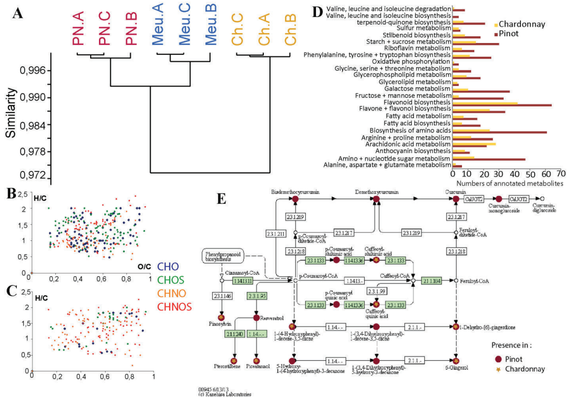
Figure 2: FTICR-MS data for single variety wines (vintage 2008). (A) Hierarchical cluster analysis of spectra from Pinot noir wines (red) Pinot Meunier wines (blue) and Chardonnay wines (yellow), showing the higher similarity between the two Pinots. (B) van Krevelen diagram (H/C versus O/C) of specific masses for Pinot wines (Pinot Noir and Meunier). (C) van Krevelen diagram (H/C versus O/C) of specific masses for Chardonnay. (D) Comparison of the number of possible Pinot (red) and Chardonnay (yellow) metabolites annotations in the various metabolic pathways of the Vitis vinifera organism. (E) Comparison of Pinot (red discs) and Chardonnay (yellow stars) possible annotations in the stilbenoids biosynthesis pathway.
