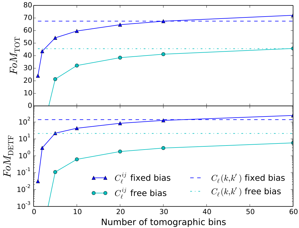
Figure 10.2: Comparison of the total FoM_{TOT} (top) and dark energy FoM_{DETF} (bottom) figures of merit for the 3D Fourier-Bessel analysis (horizontal dashed lines) vs. tomographic analysis (solid lines) as a function of number of redshift bins. The upper lines (dashed and triangle) result from assuming a fixed bias, the lower lines (dotted and circle) are obtained when assuming a grid of 5 \times 5 nuisance parameters in scale and redshift described in Section 10.3.1.5.
