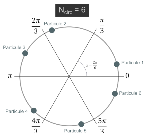
FIGURE 3.11 – Splitting circulaire
