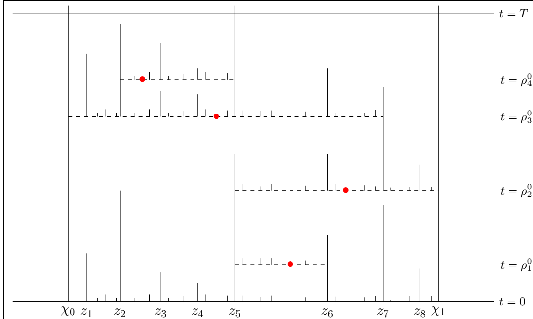
Figure III.2.: LFF( \beta )–process with \beta \in (0, \infty) .
