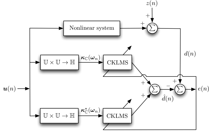
Figure 5.3: Block diagram of ACKLMS algorithm.
