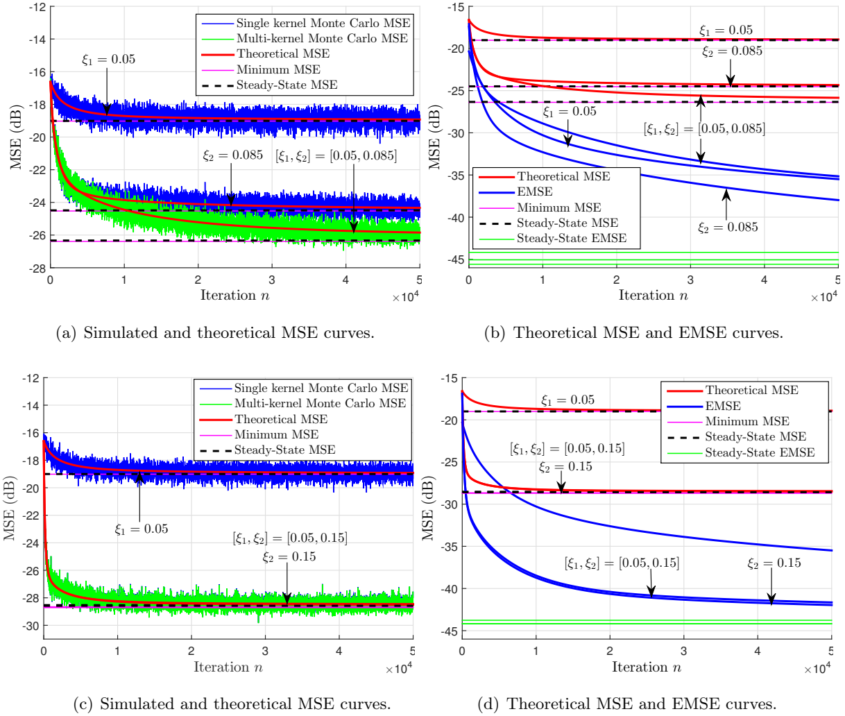
Figure 4.6: Learning curves of MI-MKLMS algorithm for Example 2 ( \xi_1 = 0.05 , \xi_2 = 0.085 for (a) and (b); \xi_1 = 0.05 , \xi_2 = 0.15 for (c) and (d)).
