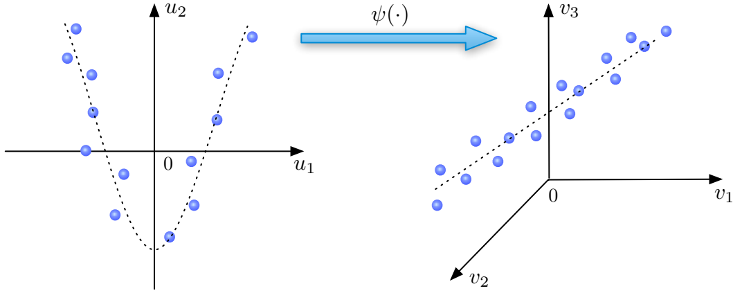
Figure 2.3: Example of nonlinear regression problem solved in a feature space with the linear method.
