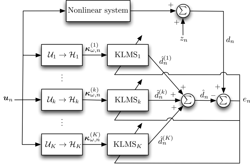
Figure 4.2: Multiple-input multikernel LMS algorithm.
