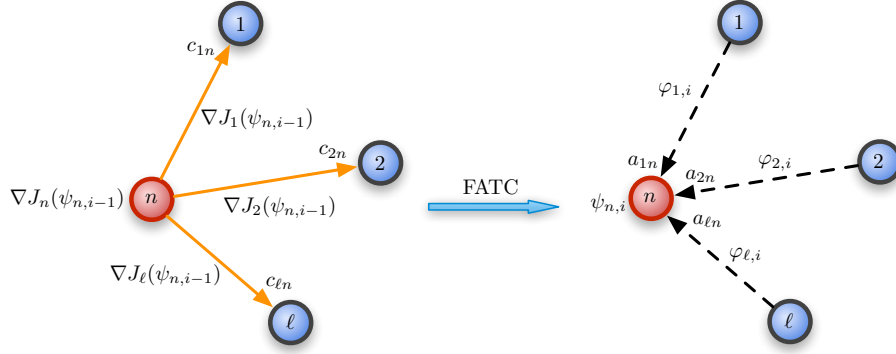
Figure 6.2: The scheme of FATC diffusion algorithm.
