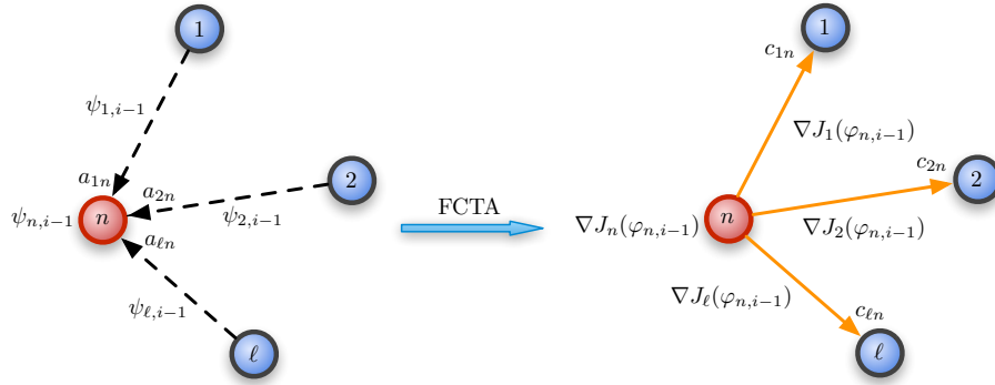
Figure 6.3: The scheme of FCTA diffusion algorithm.
