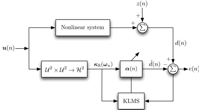
Figure 5.1: Block diagram of complexified kernel LMS algorithm.
