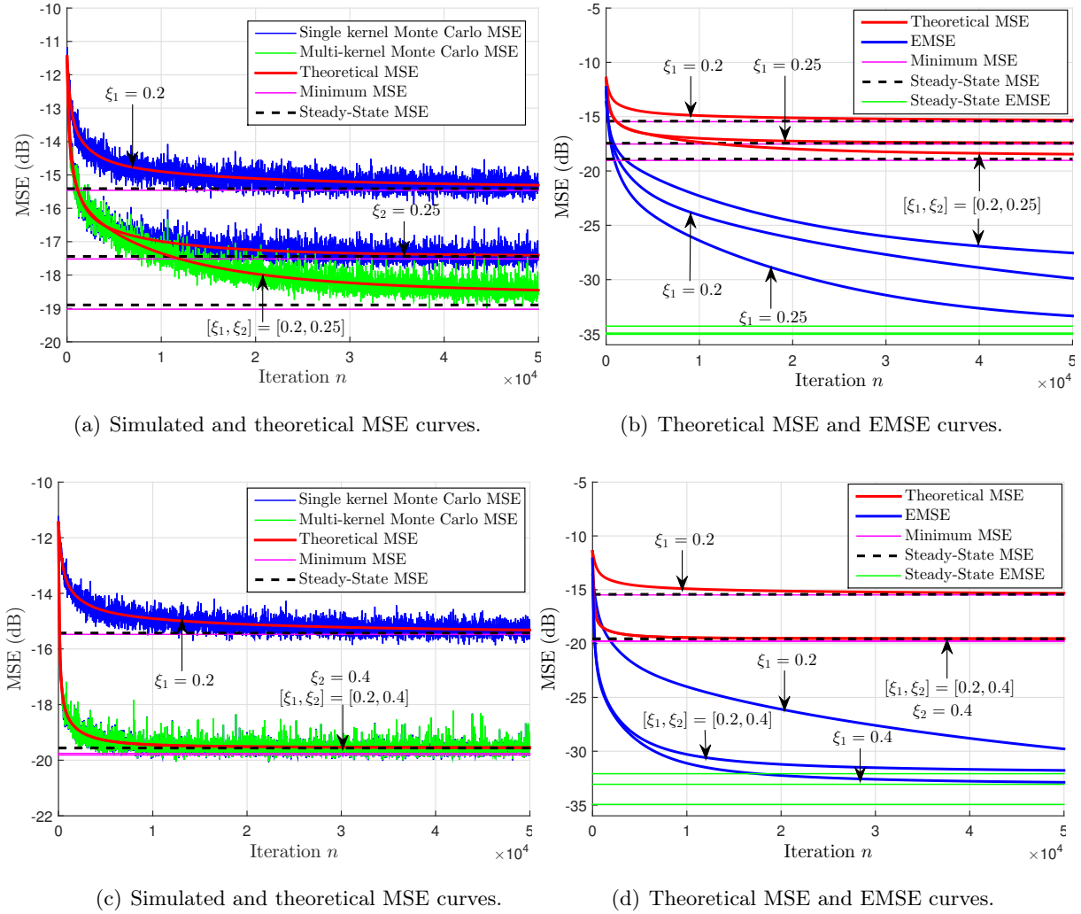
Figure 4.4: Learning curves of MI-MKLMS algorithm for Example 1 ( \xi_1 = 0.2 , \xi_2 = 0.25 for (a) and (b); \xi_1 = 0.2 , \xi_2 = 0.4 for (c) and (d)).
