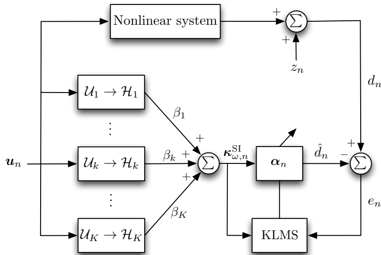
Figure 4.1: Single-input multikernel LMS algorithm.
