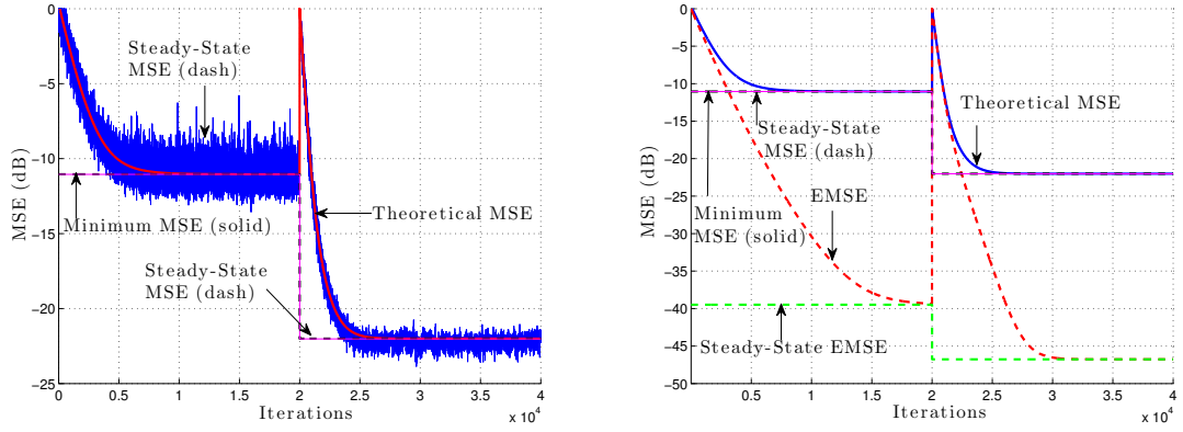
(b) \mathcal{D}_2 = \{10@0.15\}
