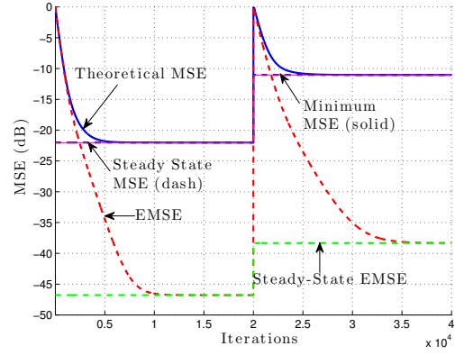
(a) \mathcal{D}_2 = \{10@0.15\}
