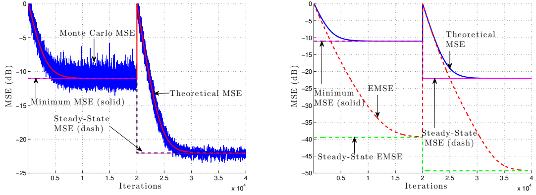
(a) \mathcal{D}_2 = \{10@0.35\}
