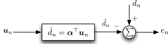
Figure 2.2: Block diagram of statistical filtering problem.
