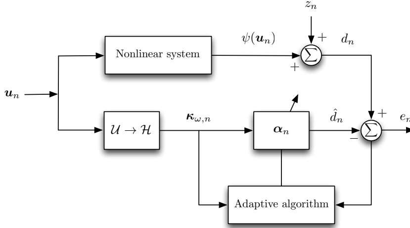
Figure 2.4: Kernel-based adaptive system identification.
