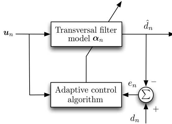
Figure 2.1: Block diagram of linear adaptive filter.
