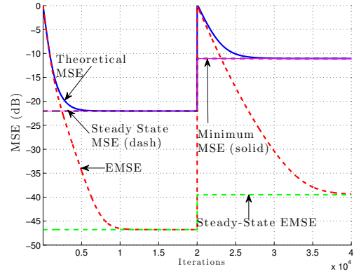
(b) \mathcal{D}_2 = \{10@0.35\}
