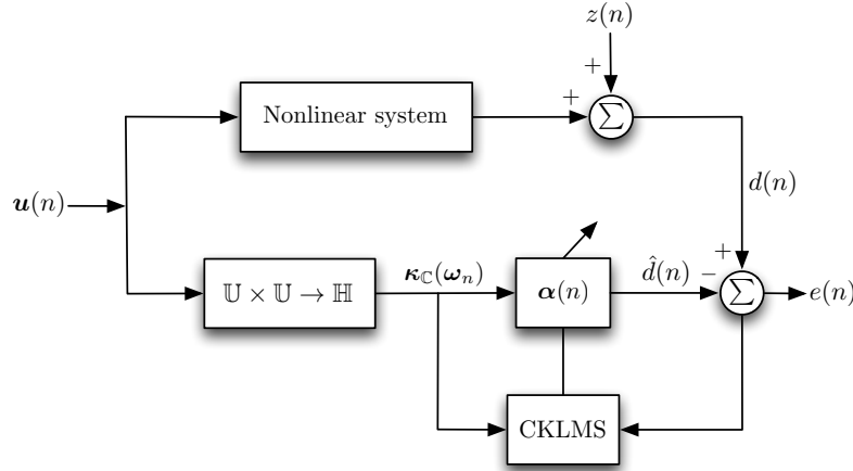
Figure 5.2: Block diagram of pure complex kernel LMS algorithm.
