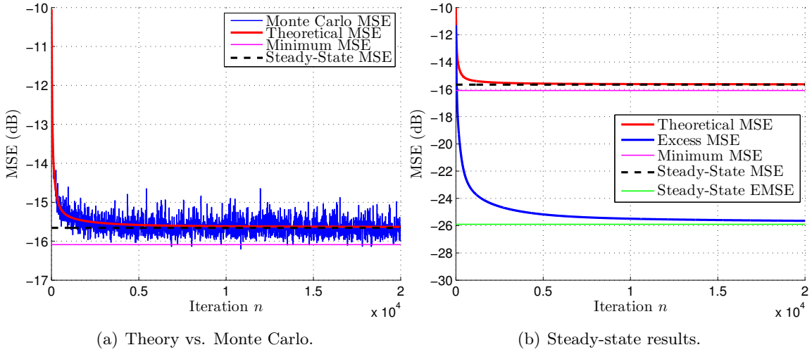
Figure 5.4: Simulation results of ACKLMS algorithm ( \rho = 0.1 , \xi = 0.55 , \eta = 0.1 and M = 12 ).
