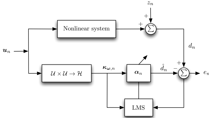
Figure 3.1: Monokernel LMS adaptive filtering.
