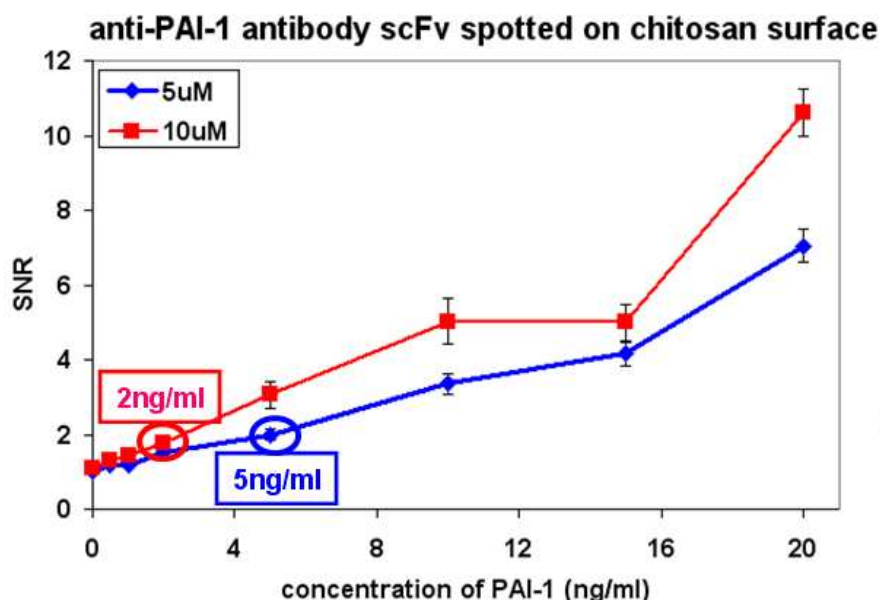
Figure 9 Detection of PAI-1 on chitosan surface, as a function of anti-PAI-1scFv spotted (5 \mu M and 10 \mu M); limit of detection (LOD) of PAI-1 for each concentration was indicated.
