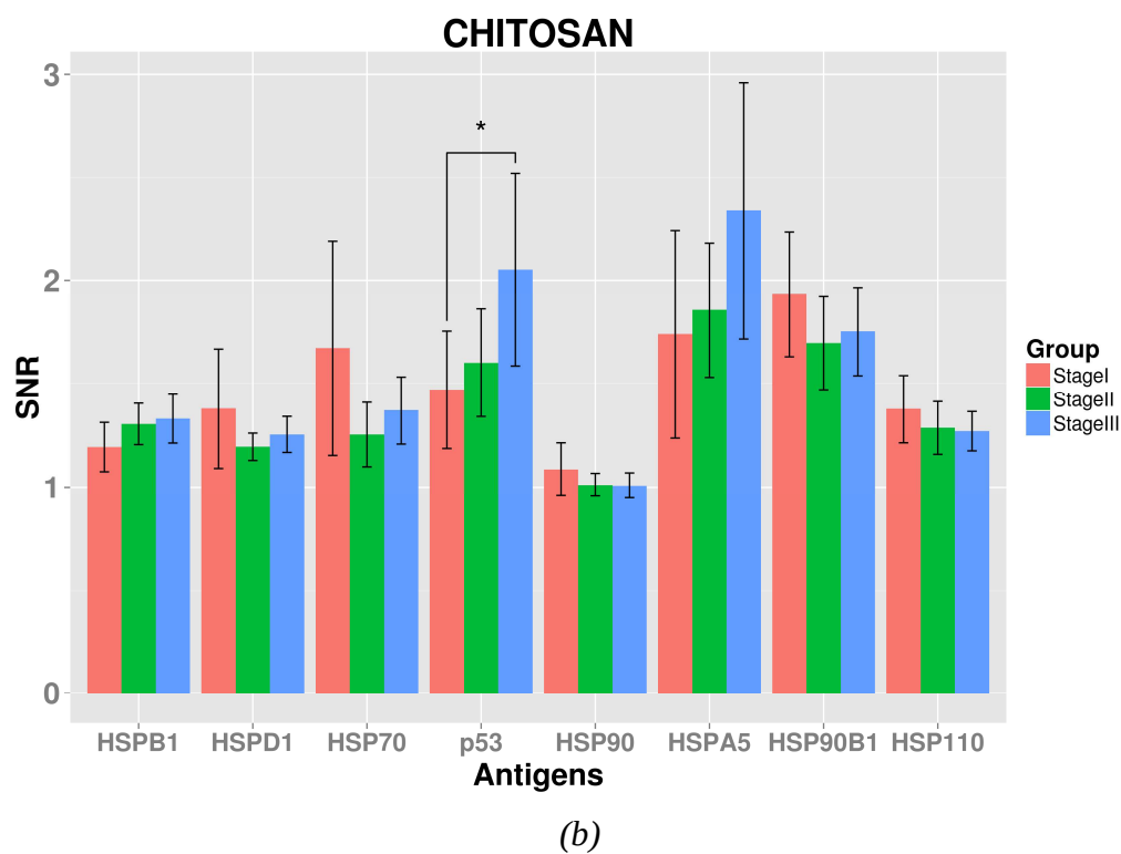
Figure 10 Correlation between the presence of autoantibodies against HSPs and P53 with tumor stage obtained on COOH(a) and chitosan (b) surfaces; *: p < 0.05 ( p value was calculated by Mann–Whitney test).
