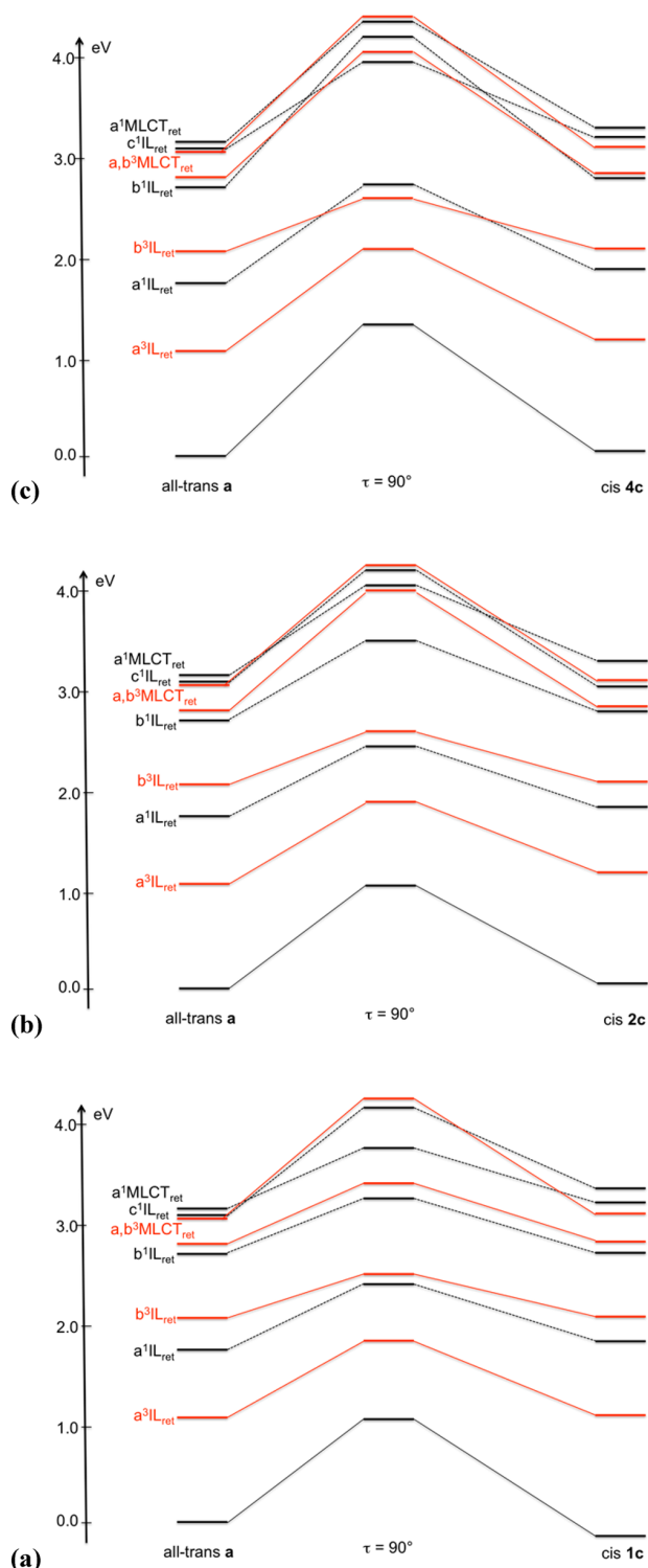
Figure 3. TD-DFT state correlation diagrams connecting the low-lying singlet and triplet excited states of all- trans [Re(CO) 3 (bpy)(L)] + a to the corresponding states of the cis isomers (a) 1c , (b) 2c , and (c) 4c . (black: singlet states; red: triplet states).
