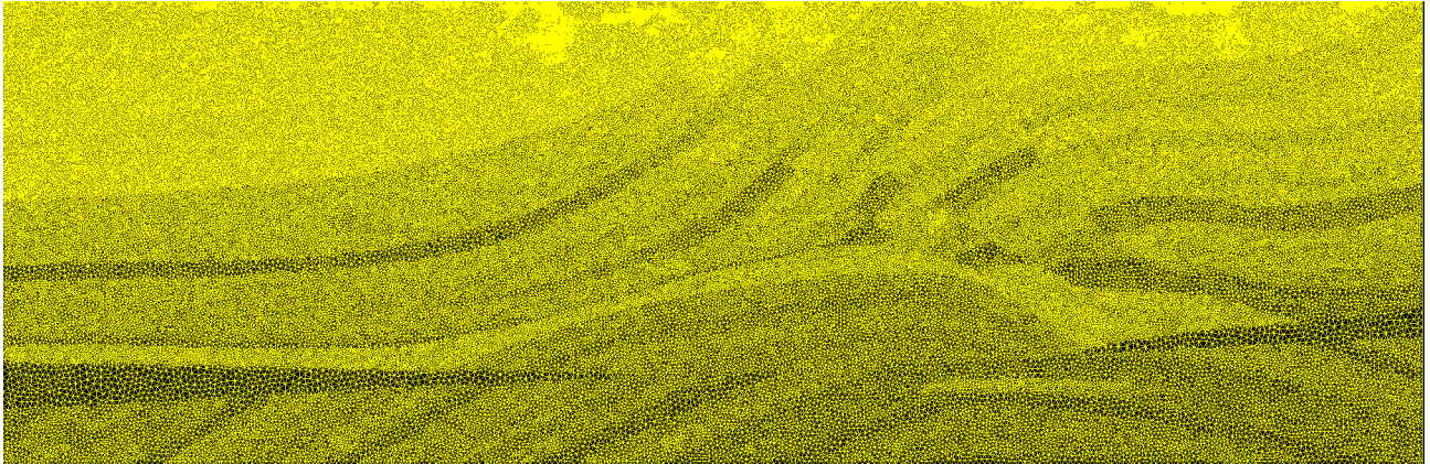
Fig. 4.5.2: Marmousi discretization.
