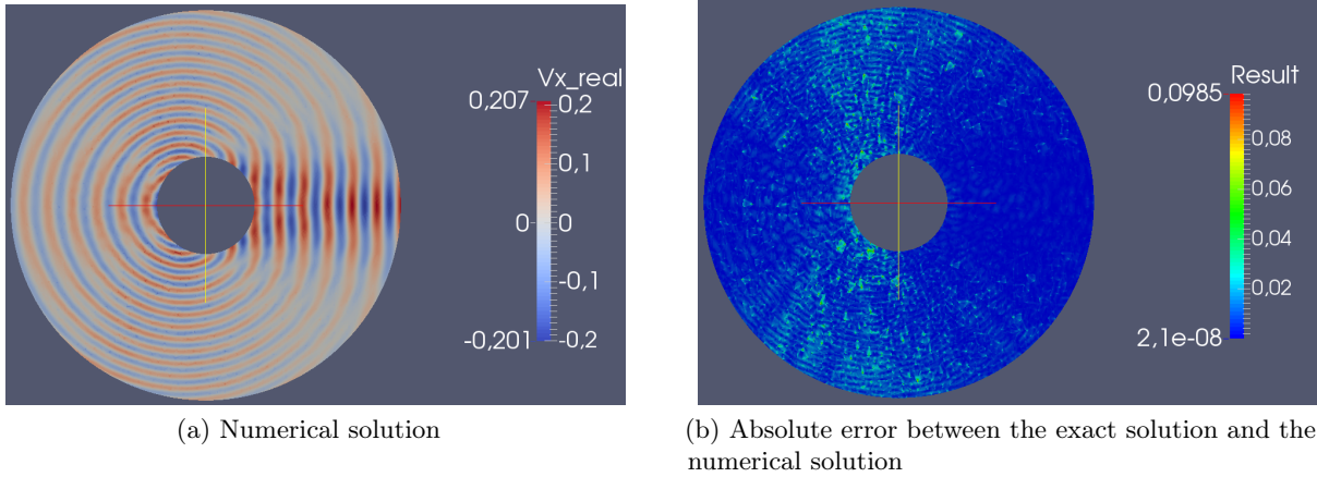
Fig. 4.3.7: Disk-shaped scatterer: numerical solution, mesh M2, HDG- \mathbb{P}_3 scheme, V_x component.
