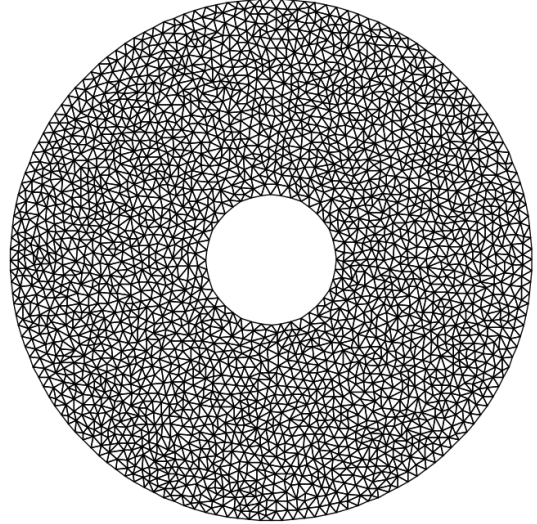
(b) Mesh M2, 5100 elements.
