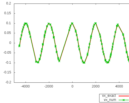
(b) Upwind flux DGFD- \mathbb{P}_2 scheme.
