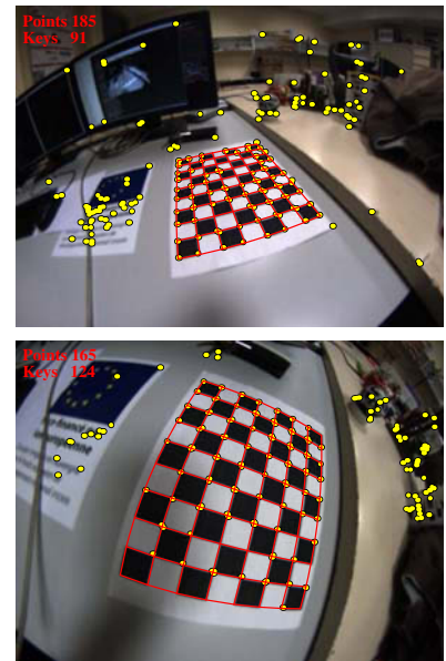
(e) MCSLAM
