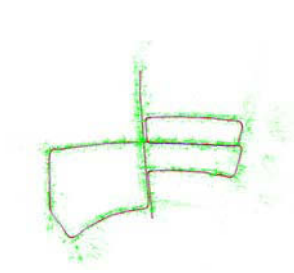
(e) Reconstruction
