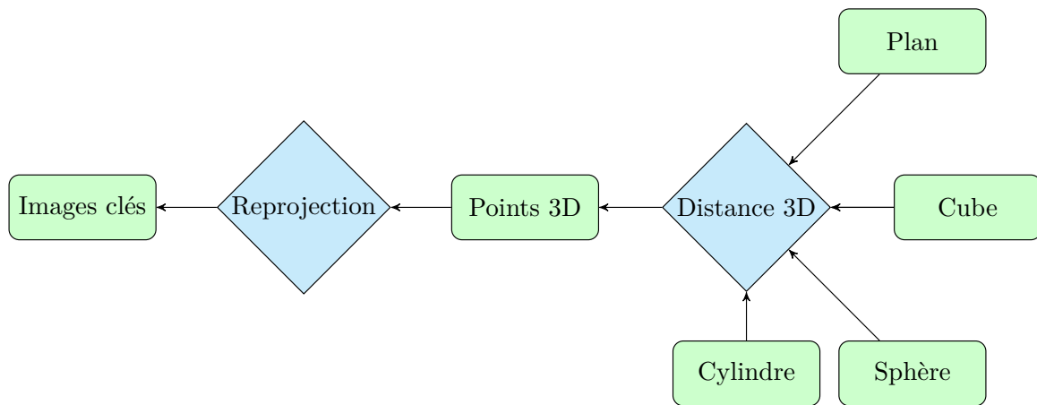
(a) Graphe
