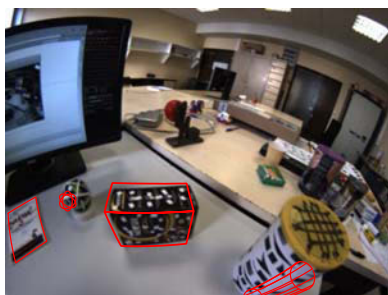
(b) SLAM
