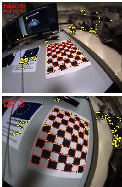
(c) SLAM
