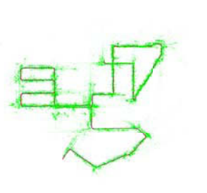
(i) Reconstruction
