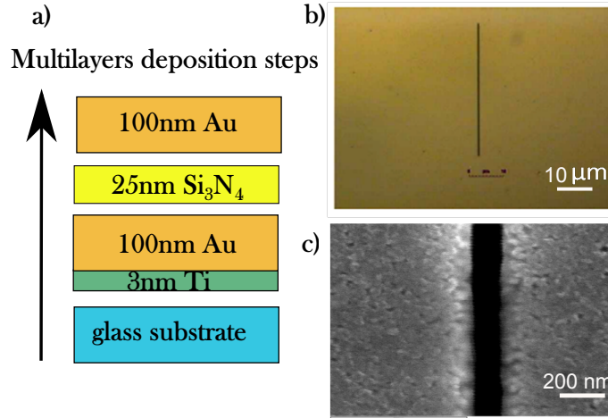
Figure 3.7: New sample design and fabrication: (a) Multilayer-ed structure of the sample. (b) Optical microscope image of a 300nm×40μm slit etched in the multilayered structure; (c) A Scanning Electron Microscope image of a nanoslit.
