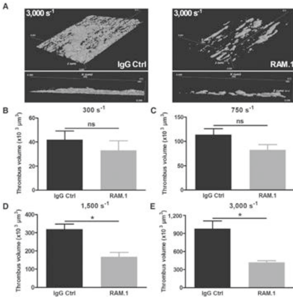
Figure 3. RAM.1 inhibits thrombus growth in an in vitro flow system. A–E , Anticoagulated mouse whole blood (hirudin: 100 U/mL) labeled with 3,3'-dihexyloxycarbocyanine iodide (1 μmol/L) and incubated with RAM.1 (20 μg/mL), or a control antibody was perfused over immobilized collagen at the indicated shear rates. Thrombus growth was monitored in real time by confocal microscopy. A , Representative 3D reconstructed images of platelet thrombi obtained after 180 s of perfusion at 3000 s -1 . B–E , Bar graphs represent the thrombus volumes measured after 180 s, and data are the mean±SEM in 3 separate experiments (* P <0.05; *** P <0.001; and ns: P >0.05). IgG indicates immunoglobulin G.
